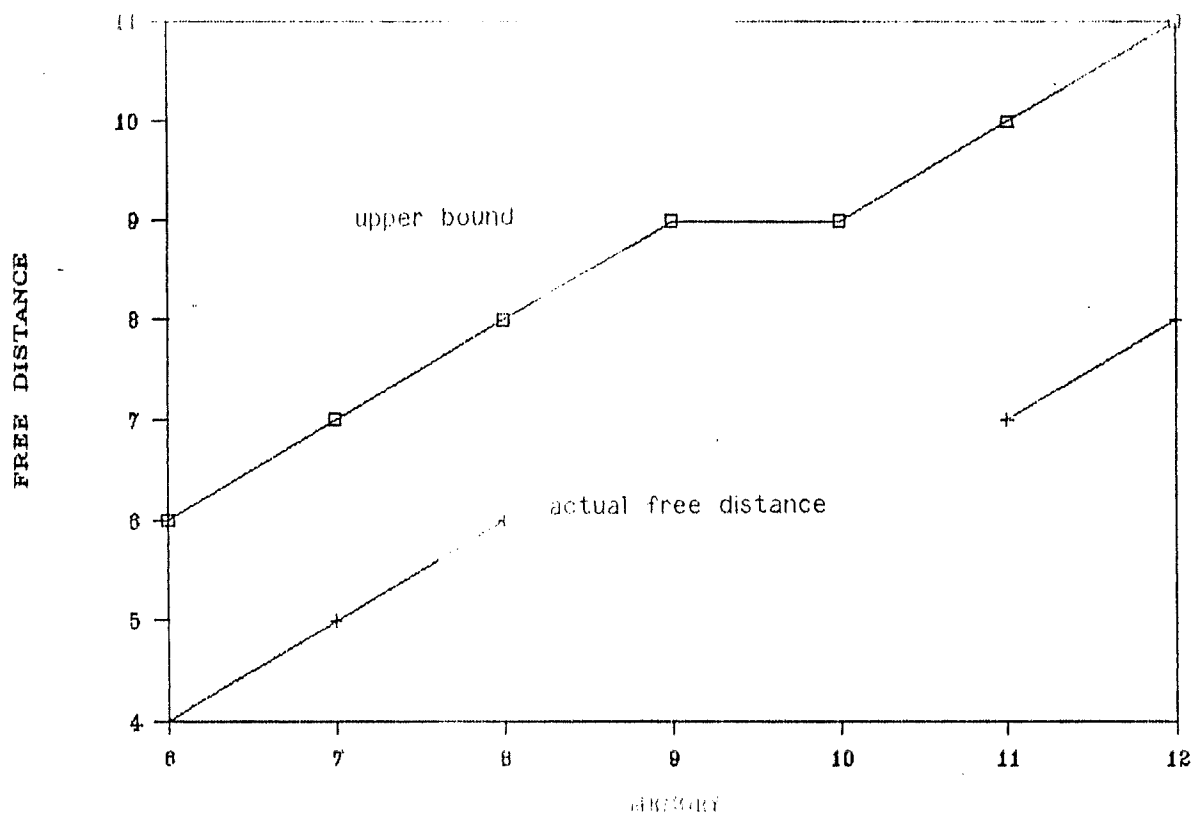
Figure 8. Free distances of some of the 2/3 codes found in comparison with the upper bound of (26), as a function of the memory.
