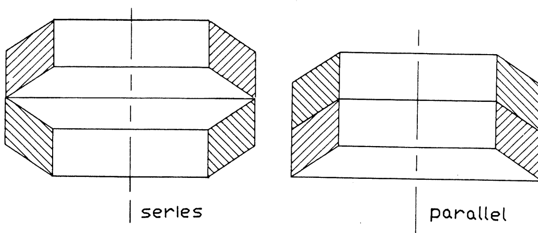
Fig. 13 Belleville springs in series and in parallel
