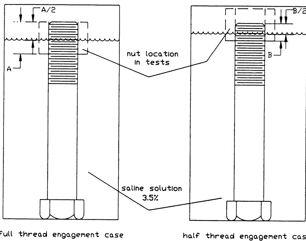
Fig. 14 Extent of immersion of bolt in saline solution for corrosion series
