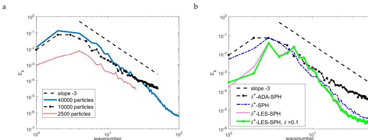
Figure 6. Inviscid two-dimensional Taylor–Green flow. Figure (a): Energy spectrum obtained using the proposed \delta^+ -ADA-SPH method with different particle resolutions . Figure (b): comparison of the results using different \delta^+ -SPH schemes using a resolution of 10,000 particles (right).
