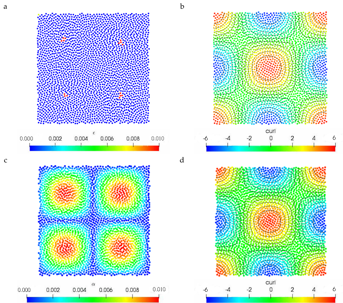
Figure 1. Two-dimensional Taylor–Green flow at Re = 100 . On the top the viscosity parameter ( \epsilon ) (a) and the vorticity field (b) obtained with the proposed \delta -ADA-SPH scheme. On the bottom we show the value of the \alpha parameter (c) and the vorticity field (d) using the \delta -LES-SPH scheme. Results obtained at t = 0.5 .
