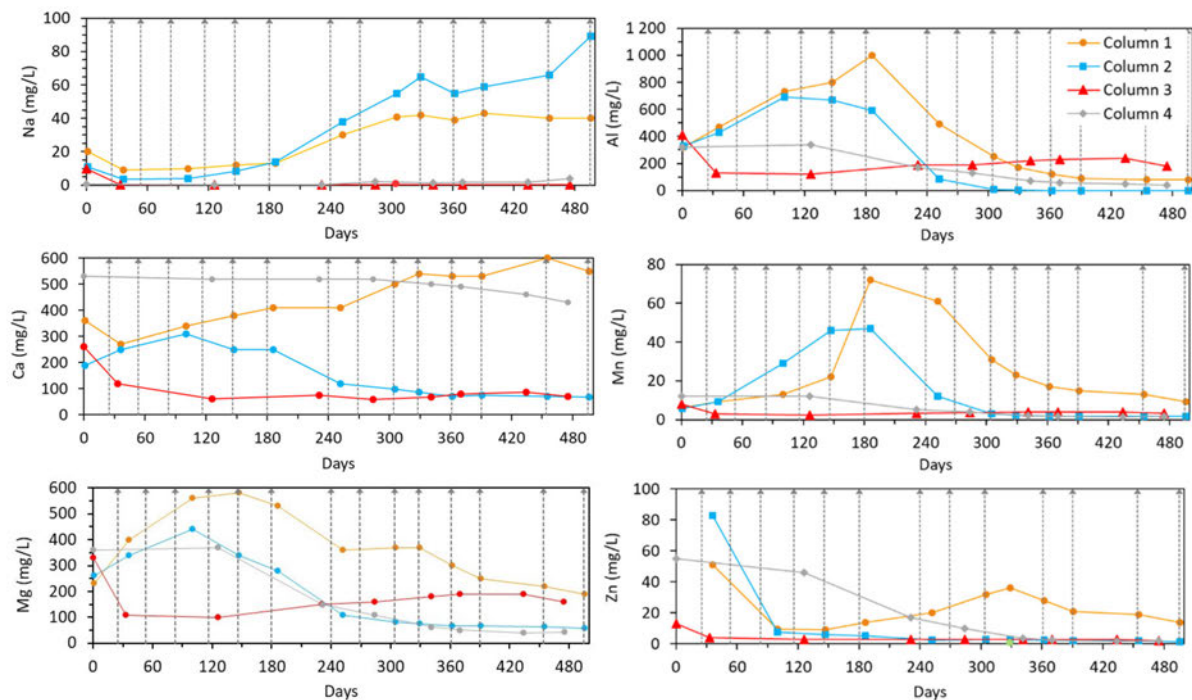
Figure 10. Concentrations of Na, Ca, Mg, Al, Mn, and Zn, as a function of time, in the column leachates. Vertical dashed lines mark the beginning of each wetting-drying cycle.
