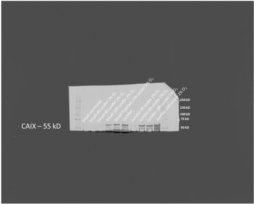
SK-LMS-1_N3_CAIX Composite
