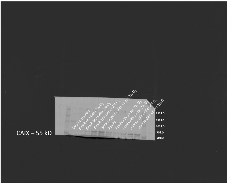
SK-LMS-1_N1_CAIX Composite
