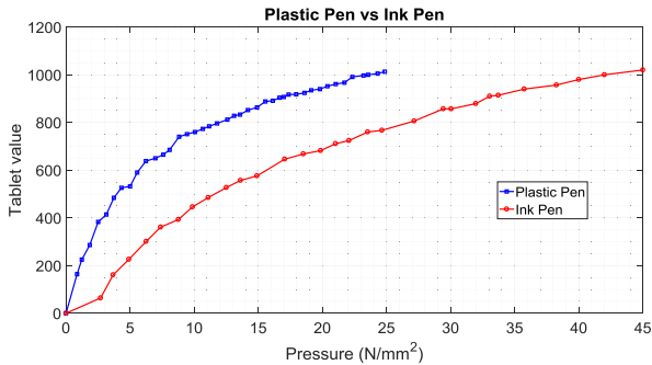
FIGURE 5. Intuos Wacom tablet value obtained for different pressure values.
