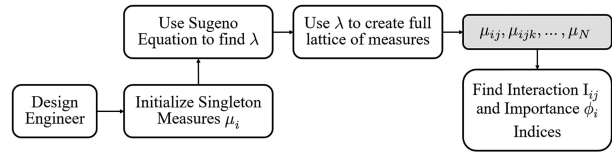
Figure 7: Identification of fuzzy measures using Sugeno process.
