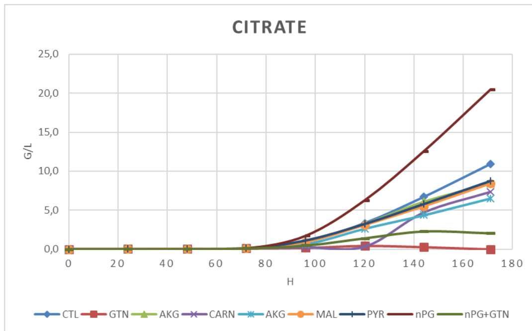
Figure SI 2: Experimental results of citrate production with addition of deferent metabolites on stat-phase. Compared to the control (CTL) condition, nPG addition stimulates citrate overproduction whereas other Krebs metabolites, \alpha -ketoglutarate/oxoglutarate (AKG), carnitine (CARN), malate (MAL), pyruvate (PYR), do not significantly change citrate production. Glutathione (GTN) addition to Y. lipolytica culture vanishes citrate production. When nPG is added jointed to GTN, citrate is produced but to a lesser extent.
