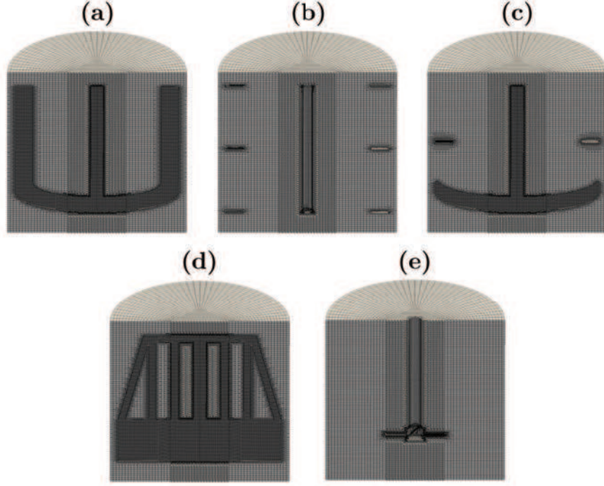
Figure 3: Illustration of the hexaedral mesh used for the (a) anchor, (b) double helical ribbon, (c) Paravisc, (d) Maxblend, and (e) PBT impellers.
