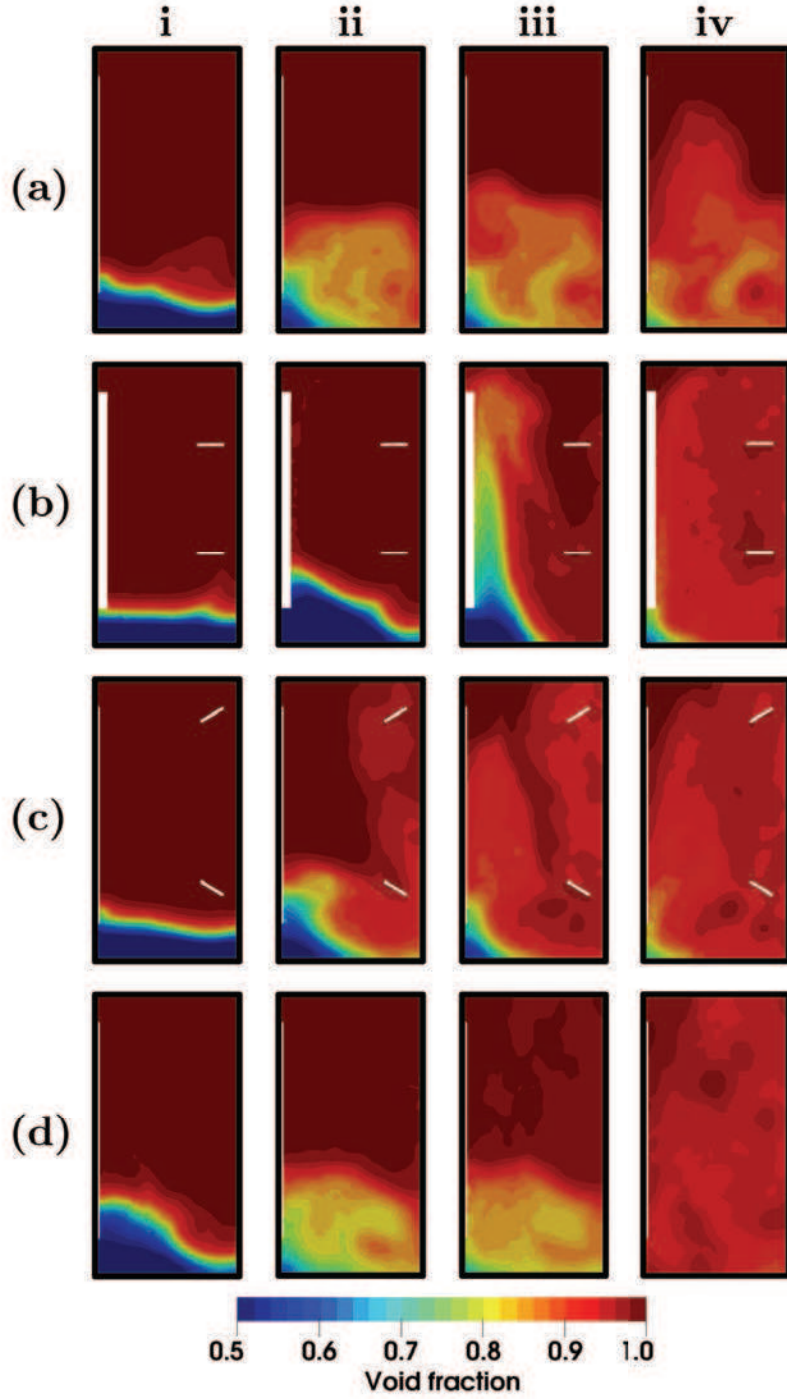
Figure 10: Void fraction profile with the (a) anchor (b) double helical ribbon (c) Paravisc and, (d) Maxblend impellers at different agitation speeds (i) N=40 RPM, (ii) N=80 RPM, (iii) N=N_{js} and, (iv) N=150 RPM. The agitation speeds (b) (iii) and (iv) for the double helical ribbon impeller are N=150 RPM and N=N_{js}=200 RPM. These results are presented when the pseudo steady-state is reached.
