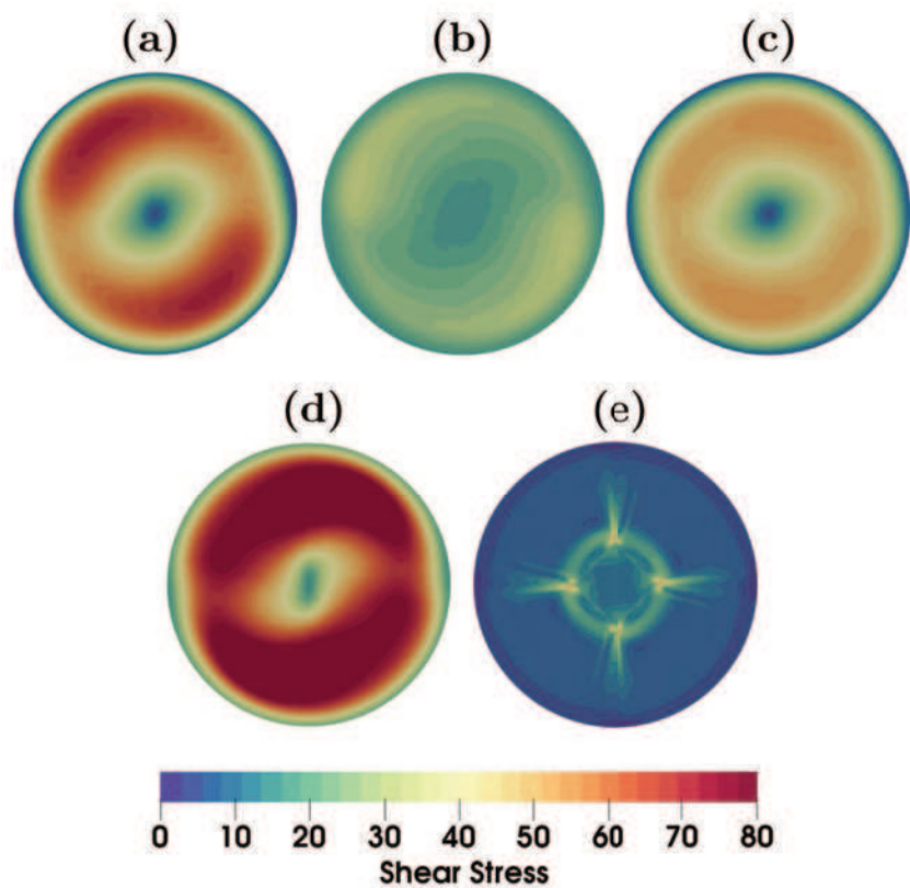
Figure 7: Visualization of the shear stresses at the bottom of the vessels ( z = 0.002cm ) generated by five single-phase mixing systems with the (a) anchor, (b) double helical ribbon, (c) Paravisc, (d) Maxblend, and (e) PBT impellers at a constant Reynolds number of Re=240 .
