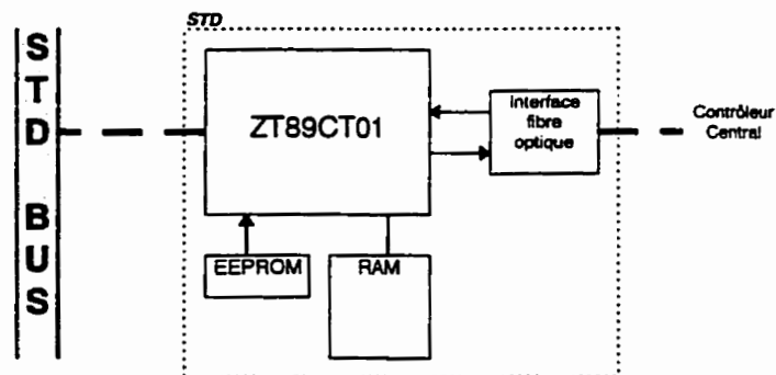
Figure 5.5: Architecture globale du STD
