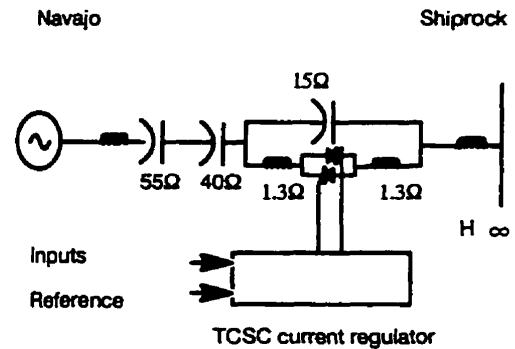
Fig. 5: Schematic diagram of Navajo-Shiprock power system with TCSC at Kayenta station
