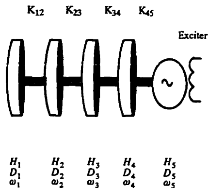
Figure 4: Schematic diagram of a synchronous machine
