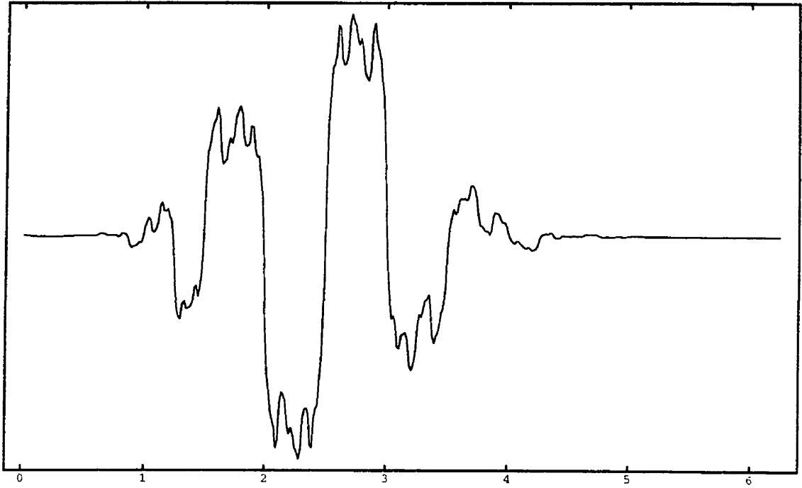
Figure 3.3: Ondelette duale {}_{3,5}\tilde{\psi}_{j,2} pour j quelconque
