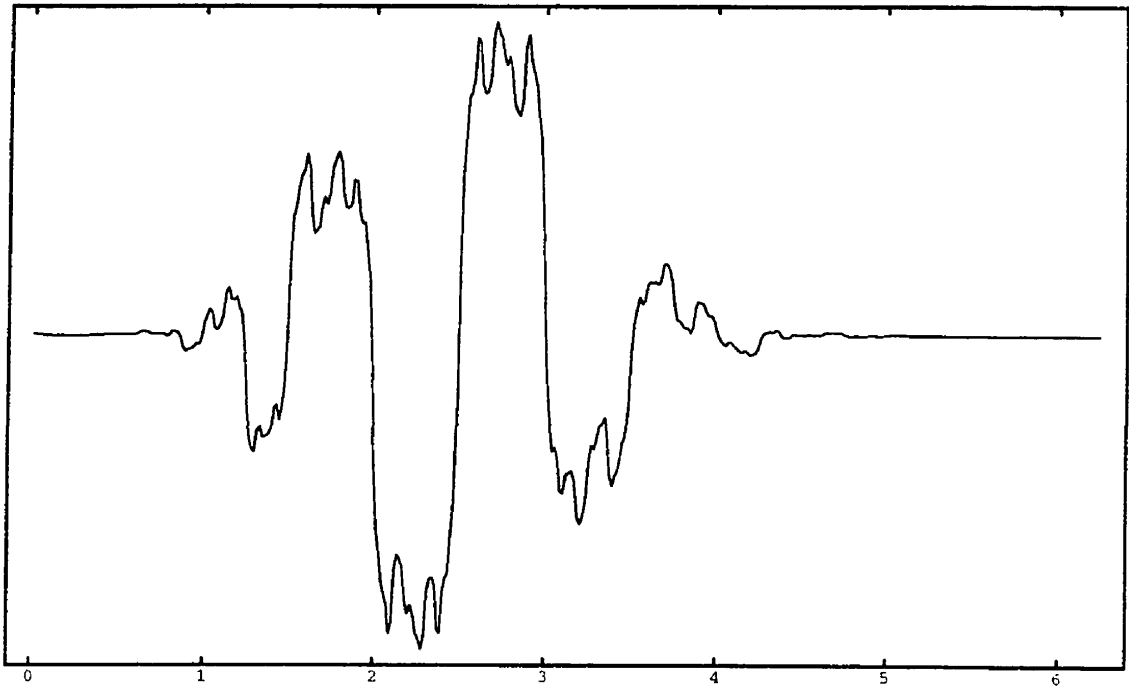
Figure 3.3: Ondelette duale _{3,5}\hat{\psi}_{j,2} pour j quelconque
