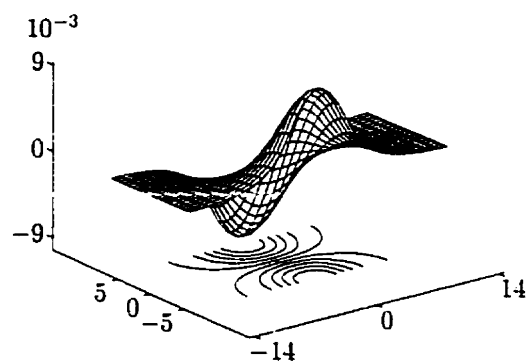
(b) H_x
