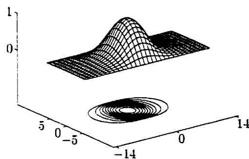
(e) E_z
