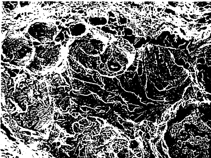
Figure 3.4 Mixture of cracking patterns in PSCC fracture ahead of the SCC crack tip in 316L stainless steel. Dimples and crystalllographic fracture appear in the austenite (A) and in the \delta -ferrite (F) respectively.
