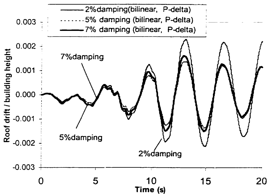
Figure 5-35 Top lateral displacement time history - scaled Saguenay earthquake (with P-Δ).
