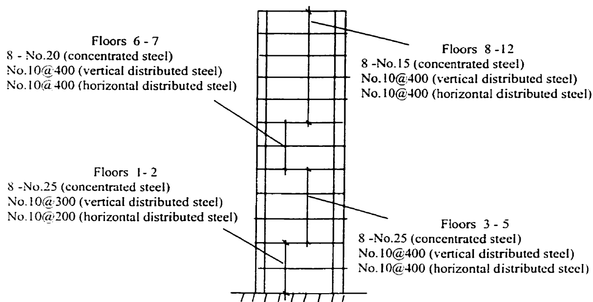
Figure 3-3 Distribution of steel along the height of the wall.
