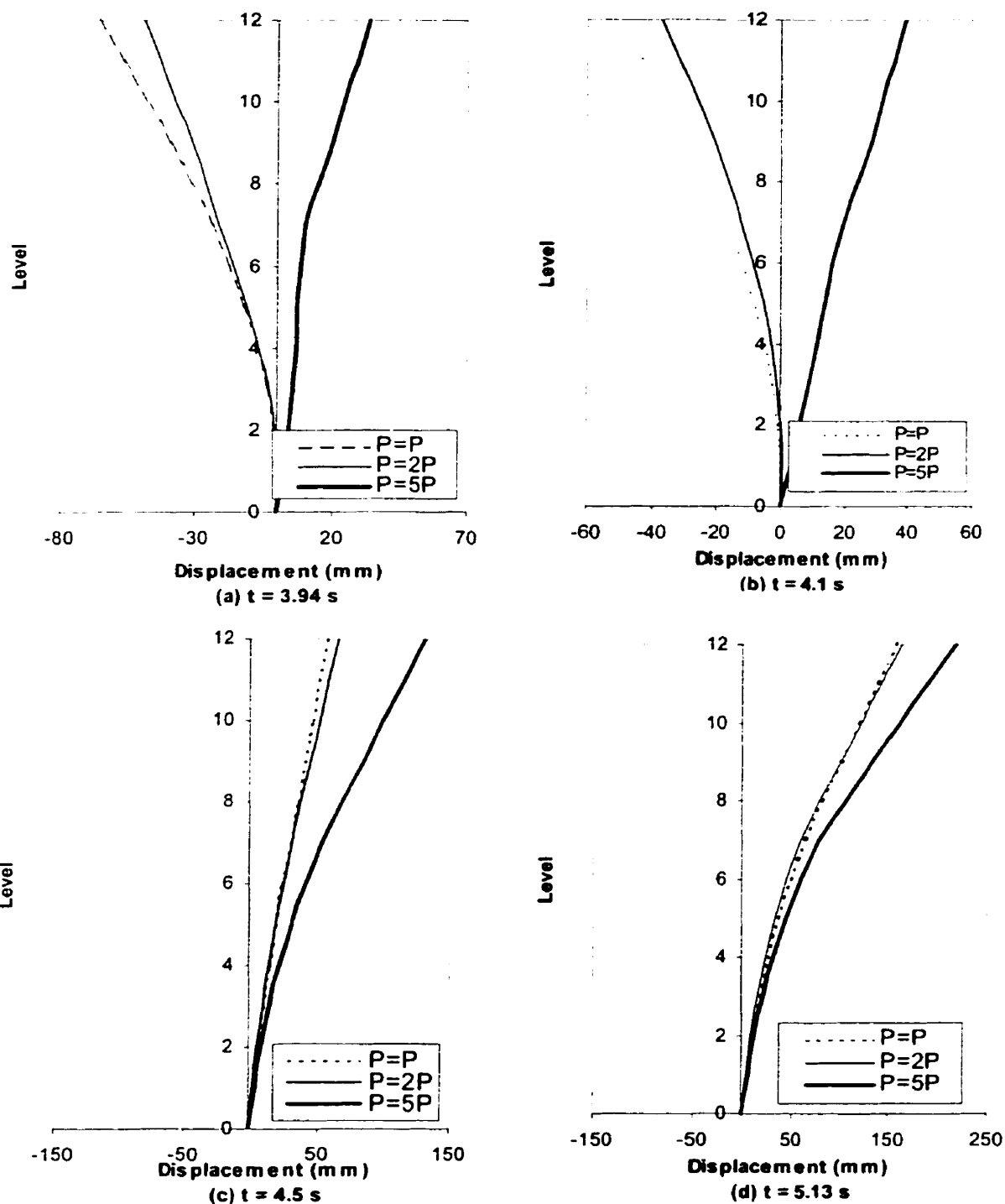
Figure 5-5 Response of the shear wall - scaled El Centro earthquake (with P-\Delta ).
