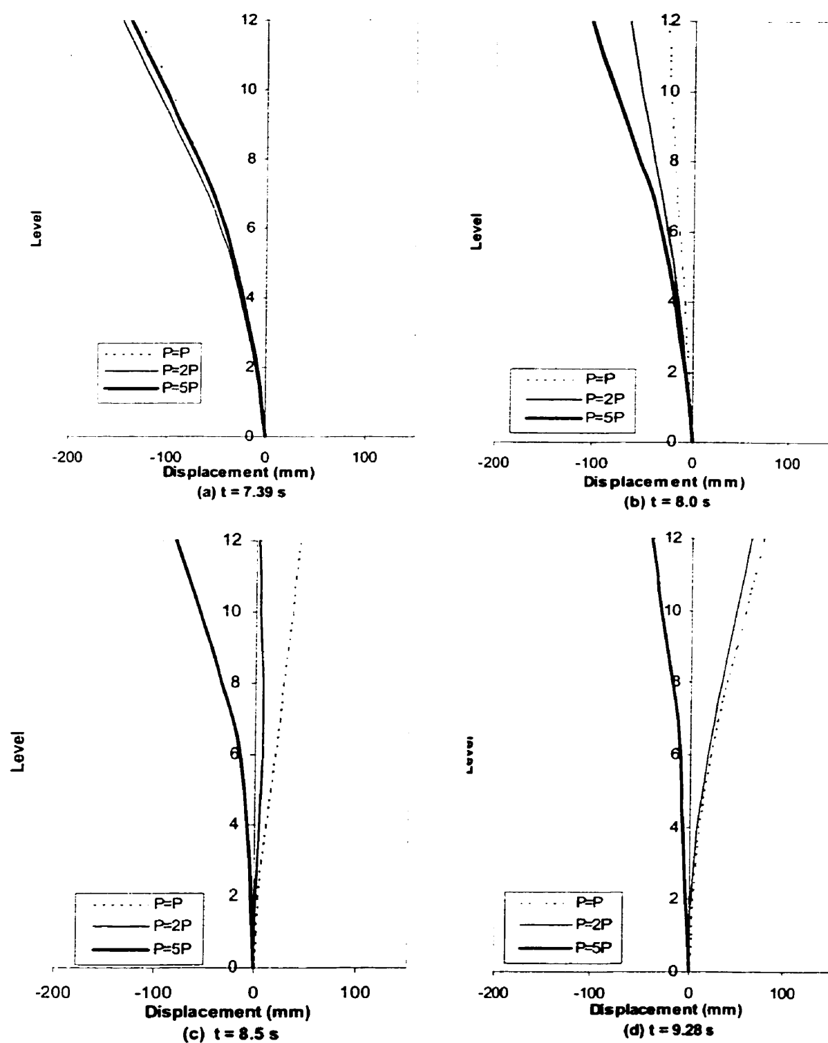
Figure S-6 Response of the shear wall - scaled Taft earthquake (with P-\Delta ).
