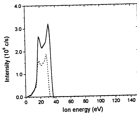
Figure 6.11 Comparison of instantaneous IEDFs from pulsed plasma (dashed lines) vs. cw plasma (solid lines): a) IEDF at a delay of 900\ \mu\text{s} (see Fig. 6.10a) compared with an IEDF from cw rf plasma ( V_b = -330\ \text{V} ); b) IEDF at a delay of 200\ \mu\text{s} compared with an IEDF from cw MW/rf plasma ( V_b = -12\ \text{V} , MW power was 300\ \text{W} ).
