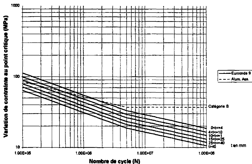
Figure 3-4 : Courbe S_{h,1} -N
