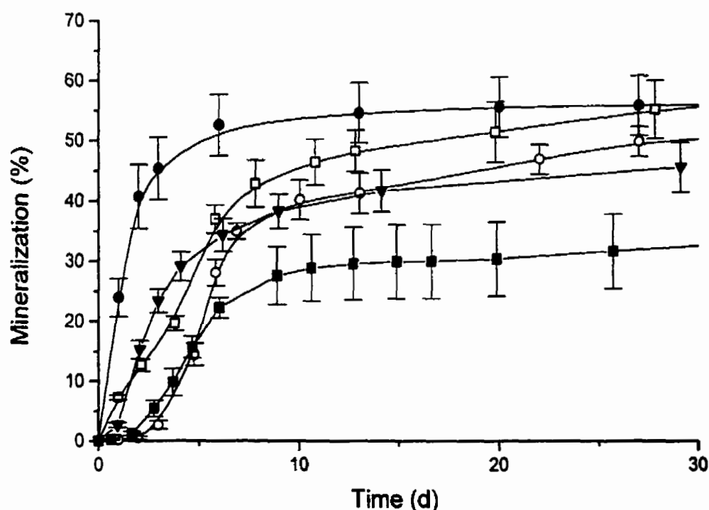
Figure 4.3: Mineralization of n -hexadecane in samples from different stages of composting contaminated soil. From the mesophilic stage (○); from the mesophilic stage (repetition) (●); from the thermophilic stage incubated at ambient temperature (□); from the thermophilic stage incubated at 55°C (●); and from the curing stage (▼). Error bars indicate the standard error (n=3). Hexadecane can be readily mineralized throughout all composting stages.
