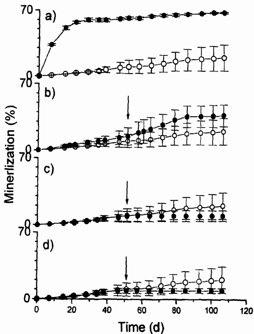
Figure 5.1: Mineralization of pyrene in contaminated soil amended with mature composted PAH-contaminated soil or fractions thereof: a) mature composted PAH-contaminated soil, b) humic acids fraction, c) fulvic acids fraction, and d) humic and fulvic acids fractions. Hollow symbols represent unamended contaminated soil. Error bars indicate standard errors (n=3). Arrows indicate addition of nine times the initial concentration.
