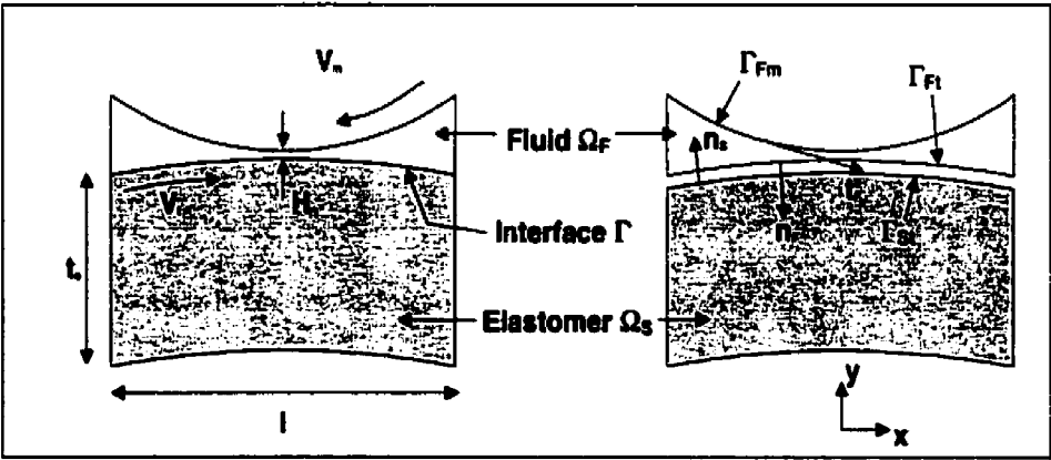
Figure A7.2 Nomenclature of the computational domain.
