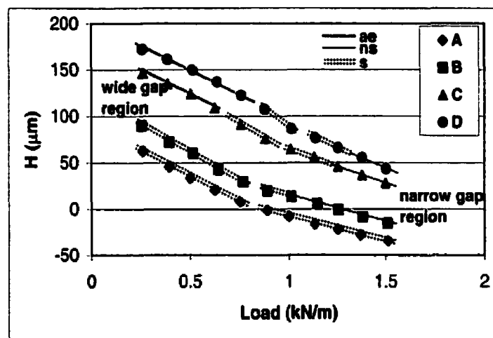
Figure 5.6(a) Apparent nip gap as function of the load on the metering rod (s = spitting present, ns = no spitting, and ae = air entrapment).
