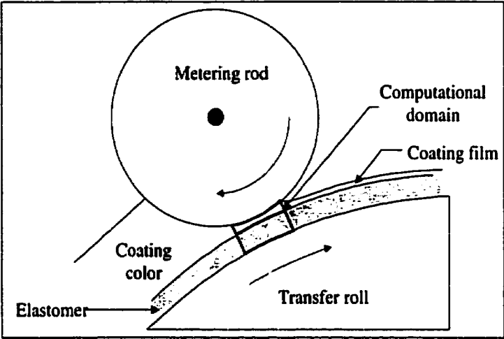
Figure A7.1 Computational domain in the simulation of the metering nip.
