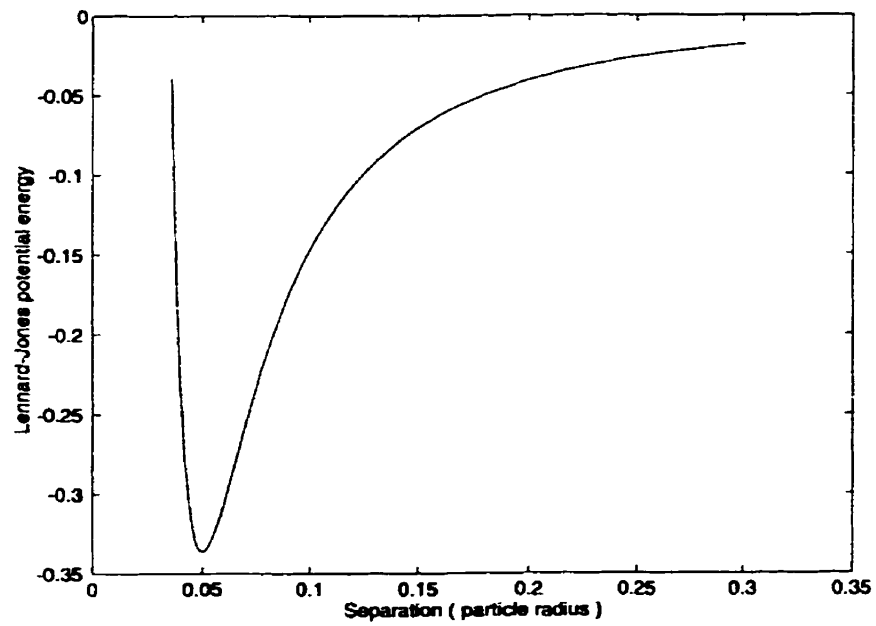
Figure 2.2 Lennard-Jones Potential
