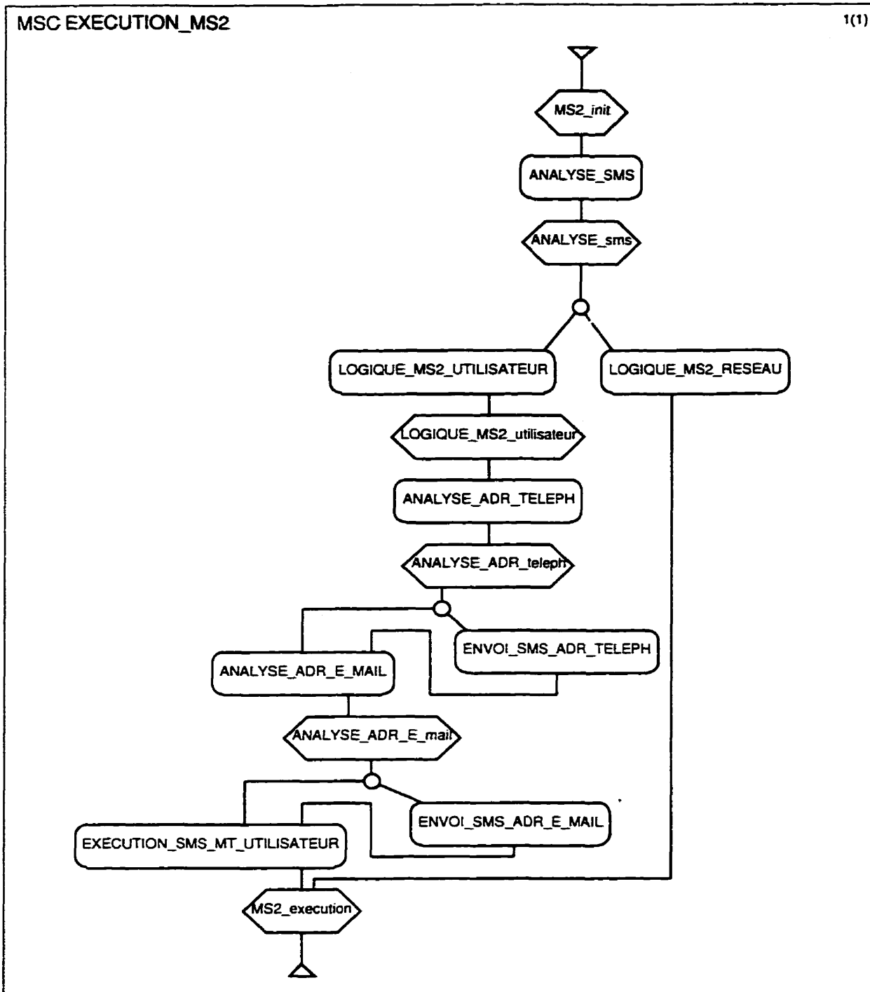
Figure B.12 : Le diagramme HMSC EXECUTION_MS2
