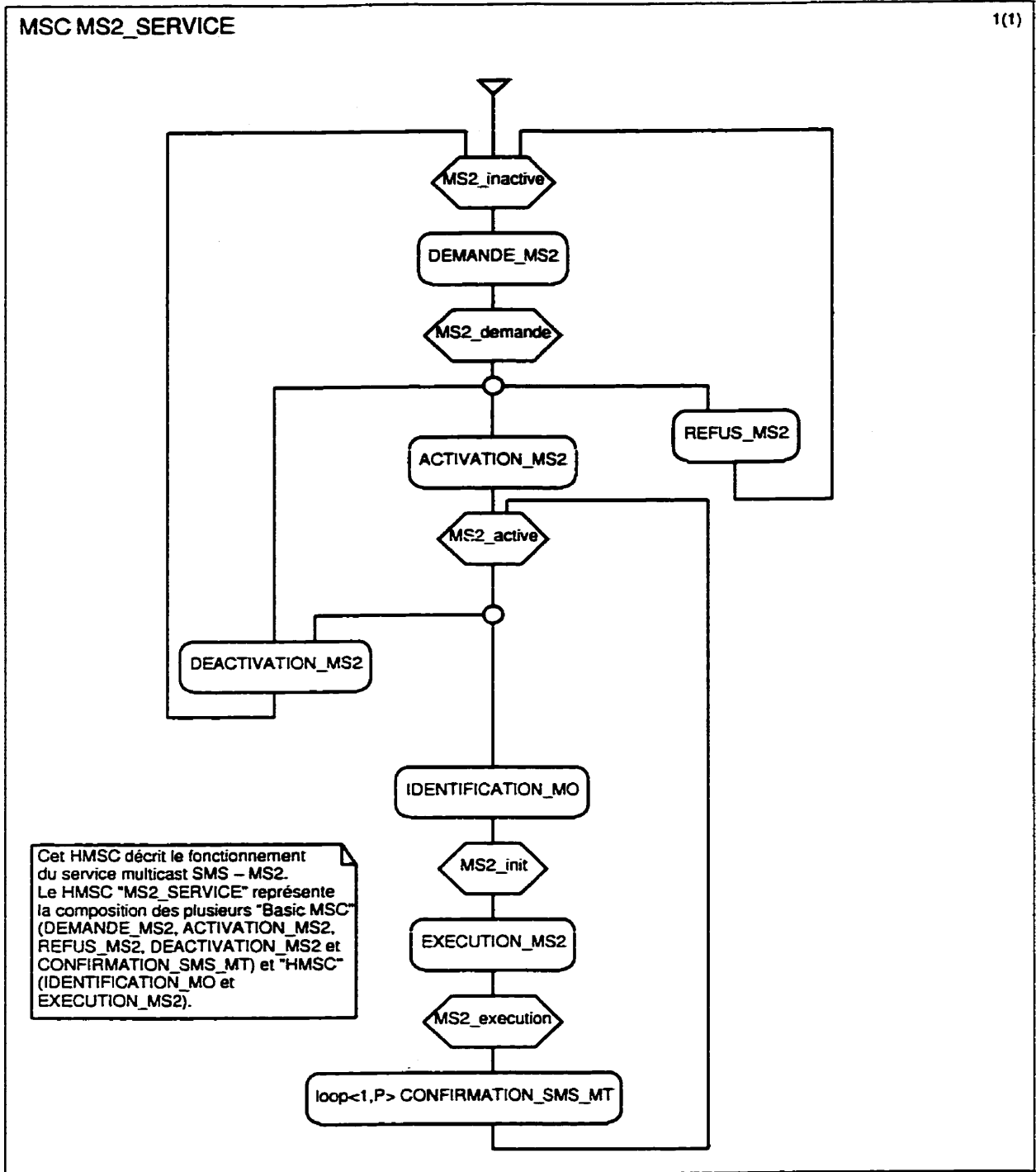
Figure 5.12 : Le diagramme HMSC MS2_SERVICE
