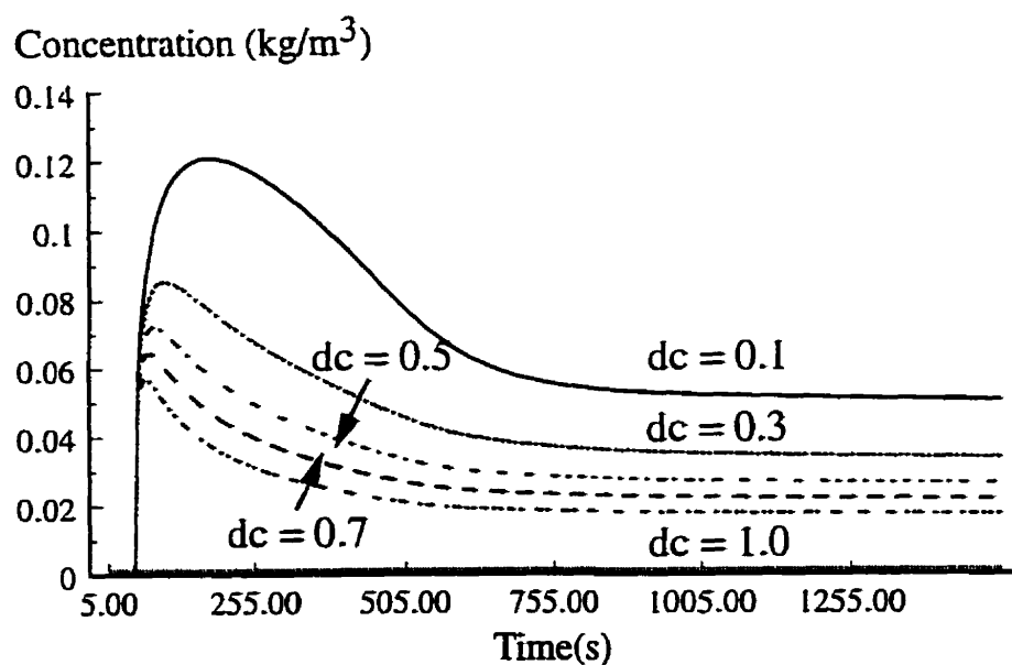
Figure 6.10 The effect of diffusion coefficient for the pollutant, with c^* = 357.5 and k = 0.00001
