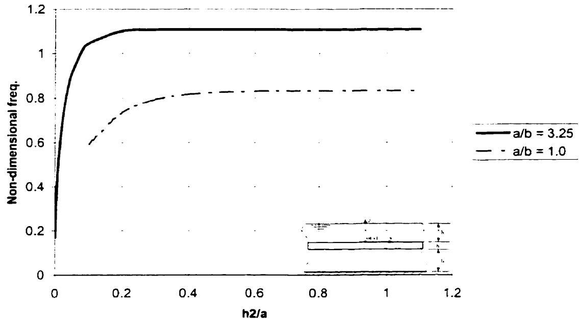
Fig. 3.8. Variation of non-dimensional first natural frequency, \Omega = \omega a^2 (\rho V/K)^{1/2} , of two cantilever plates as a function of the fluid depth h_2 .
