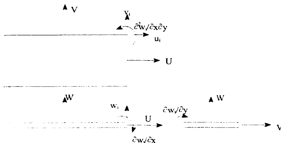
Fig. 2.3. Displacements and degrees of freedom of a rectangular plate
