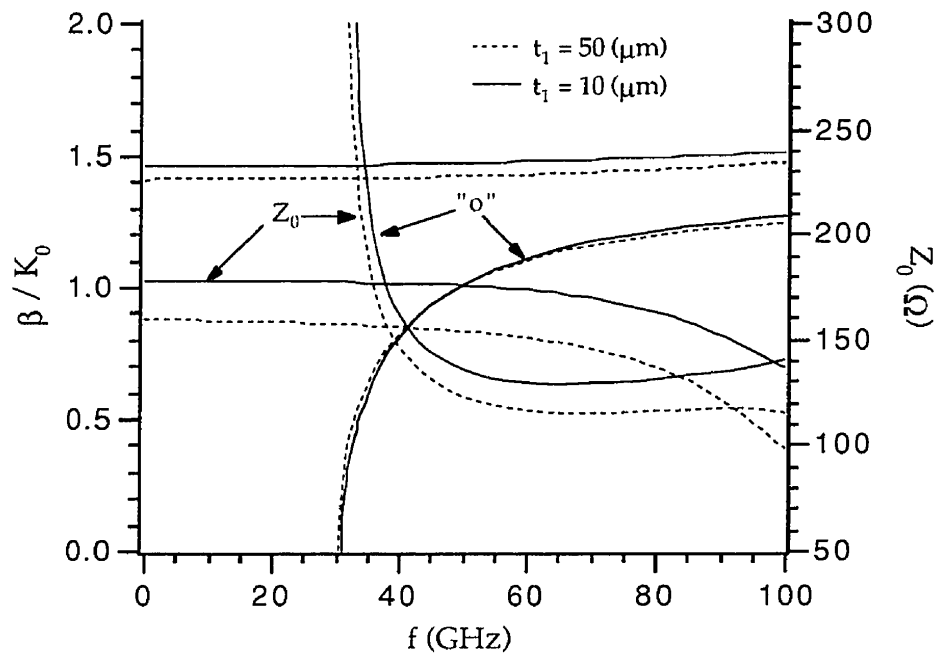
Fig. 3.7 Dispersion characteristics and characteristic impedances in coupled slotline including septum and pedestal: a = 1.55 mm, b = 1.2 mm, t_1 = t_2 , d = 0.22 mm, h_1 = h_2 = 1.39 mm, w = s = 0.2 mm, w_1 = 0.6 mm, \epsilon_r = 3.75 .
