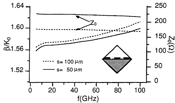
Fig. 4.8 Normalized propagation constant and characteristic impedance of the fundamental mode of a microshield line with a diamond enclosure for two widths of the central conductor and parameters are (dimensional description with respect to Fig. 4.1(f): a = 700 \mu\text{m} , h_1 = h_2 = 350 \mu\text{m} , w = 200 \mu\text{m} , t = 2 \mu\text{m} , and \epsilon_r = 4 .
