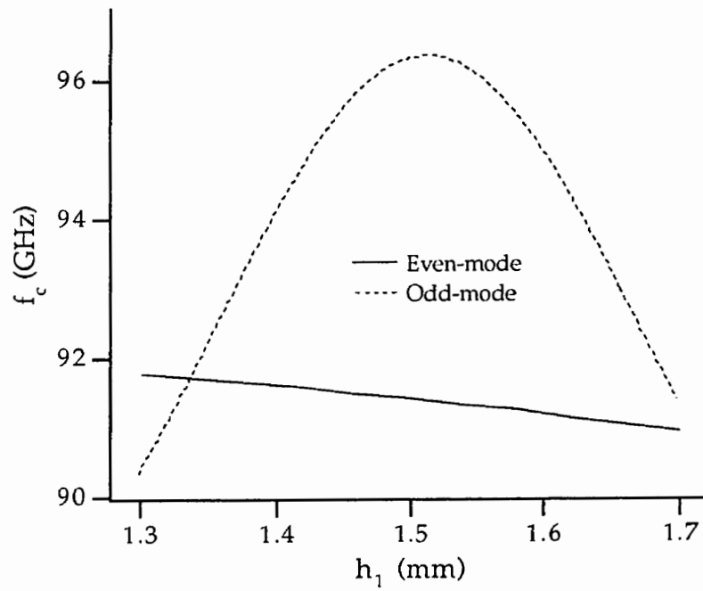
Fig. 3.5 Effect of suspended height ( h_1 ) of substrate on cutoff frequencies of the first higher-order even- and odd-modes in coupled slotline: a=b=1.55 mm, h_1+h_2=2.845 mm, w=s=0.2 mm, d=0.22 mm, t_1=35 \mu\text{m} , t_2=e=c=0 mm, \epsilon_r=3.75 .
