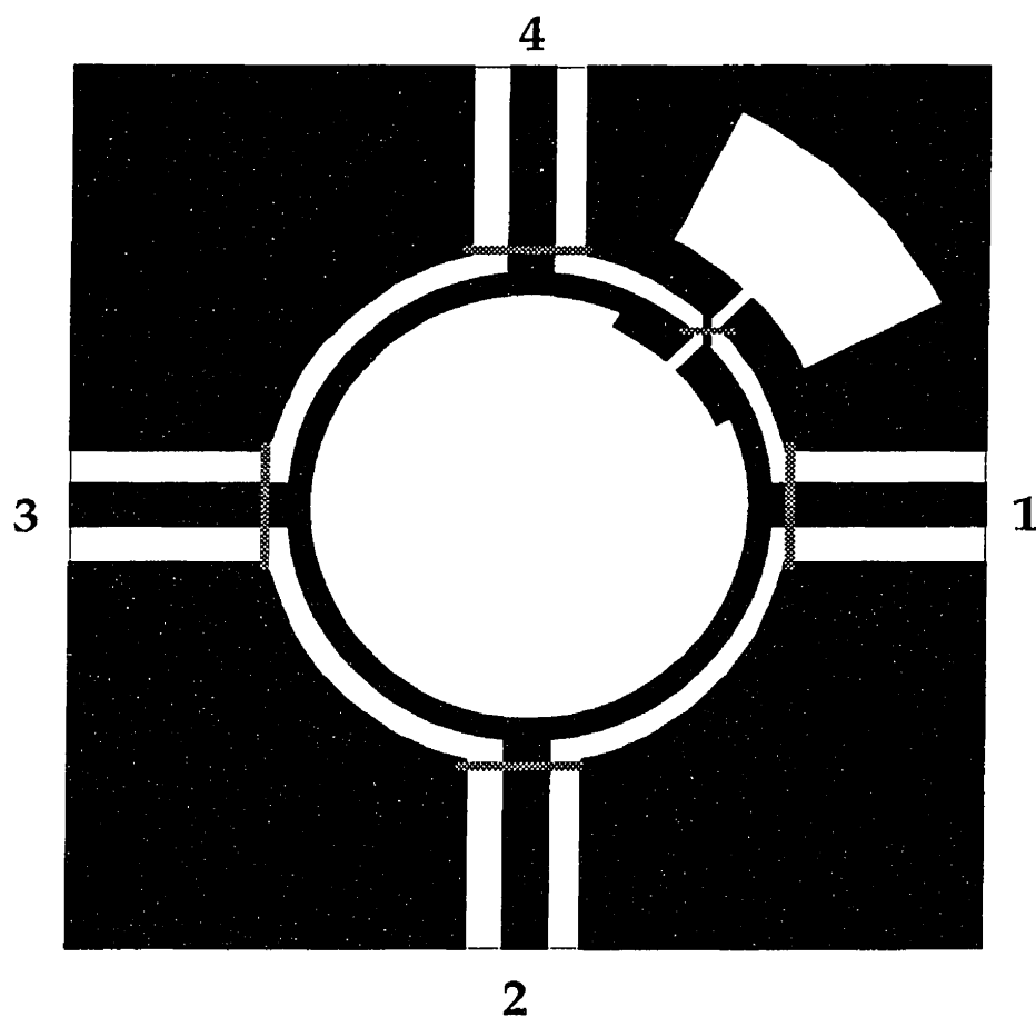
Fig. 5.11 Detailed circuit layout of a designed MCS-based hybrid ring coupler with CPS phase inverter for broadband and size-reduction experiments.
