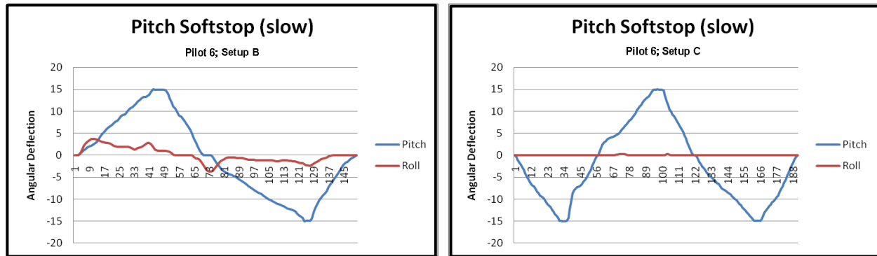
Figure 5-3 Pitch manoeuvre (slow); Pilot 6 - Setup B – no side stick skew (right) & Setup C – side stick skew (left)
