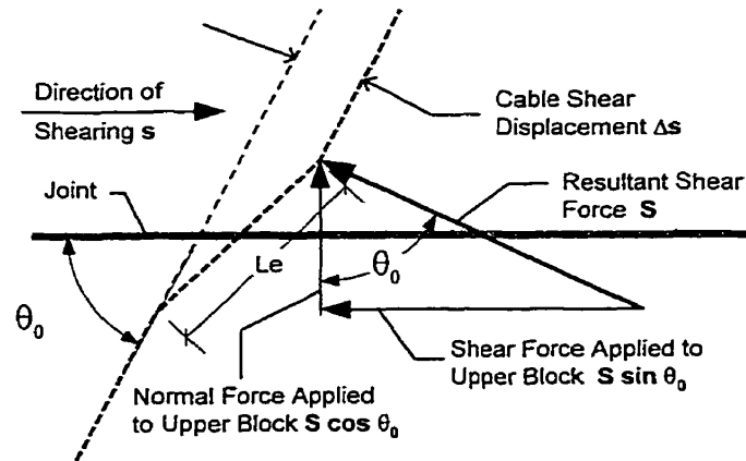
a) Shear Force Components
