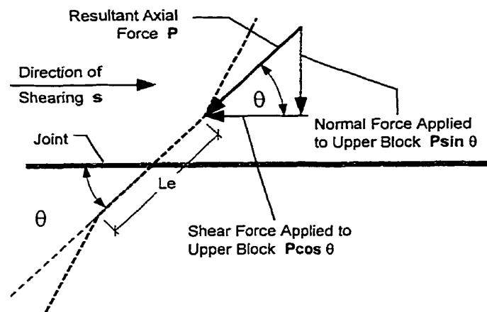
b) Axial Force Components
