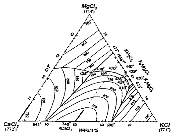
Fig. 66 - KCl-MgCl 2 -CaCl 2 system : calculated liquidus projection (wt. %).
