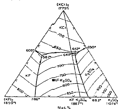
Fig. 4 - Measured K 2 Cl 2 -K 2 F 2 -K 2 SO 4 liquidus projection of Mukimov [14] .
