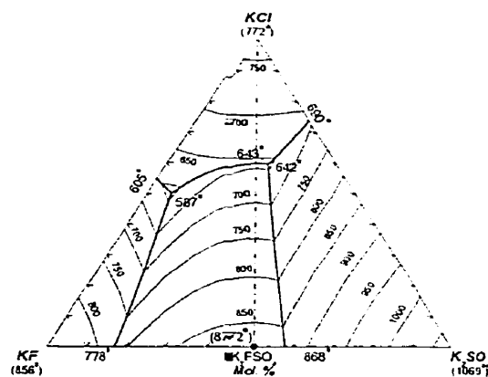
Fig. 5 - Calculated KCl-KF-K 2 SO 4 liquidus projection.
