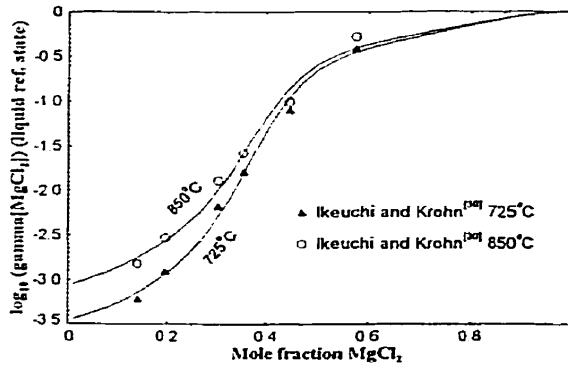
Fig. 18 - CsCl-MgCl 2 system : calculated activity coefficient of MgCl 2 in the liquid (liquid ref. state).
