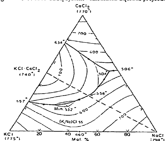
Fig. 45 - NaCl-KCl-CaCl 2 system : experimental liquidus projection of Scholich [14].
