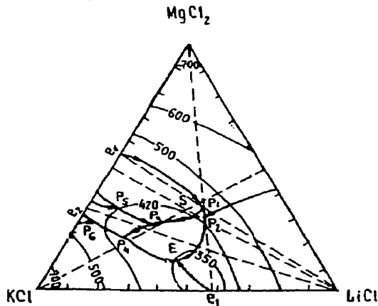
Fig. 20 - LiCl-KCl-MgCl 2 system : experimental liquidus projection of Podlesnyak et al. [47] (mol.%).
