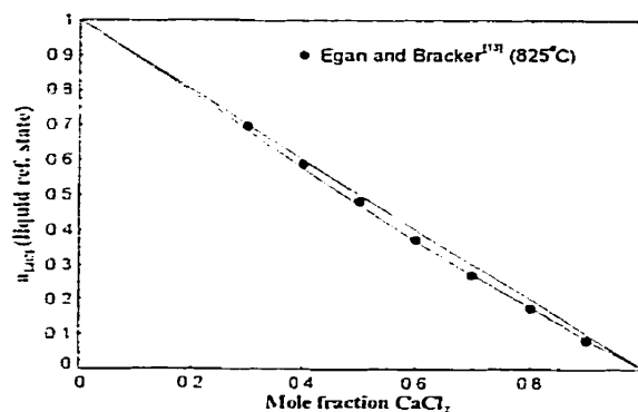
Fig. 33 - \text{LiCl-CaCl}_2 system : calculated activity of \text{LiCl} in the liquid at 825°C (liquid ref. state).
