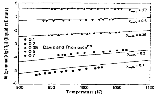
Fig. 23 - LiCl-KCl-MgCl 2 system : calculated activity coefficient of MgCl 2 in the liquid for a LiCl / (LiCl + KCl) molar ratio of 1/3 with experimental points of Davis and Thompson [49] .
