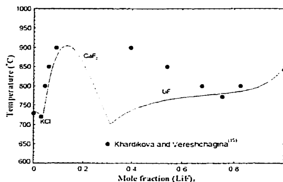
Fig. 29 - Li,K,Ca/F,Cl system: calculated [15%CaCl 2 +85%K 2 Cl 2 ]- (LiF) 2 liquids. (Labels on lines indicate the primary solid phases).
