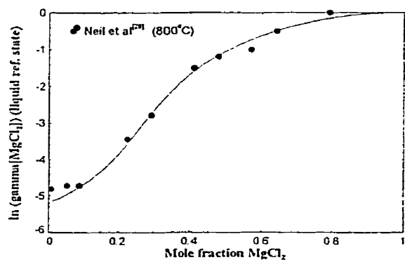
Fig. 30 - \text{NaCl-KCl-MgCl}_2 system : calculated activity coefficient of \text{MgCl}_2 in the liquid for a \text{NaCl} / (\text{NaCl} + \text{KCl}) molar ratio of 1/2 with experimental points of Neil et al. [28].
