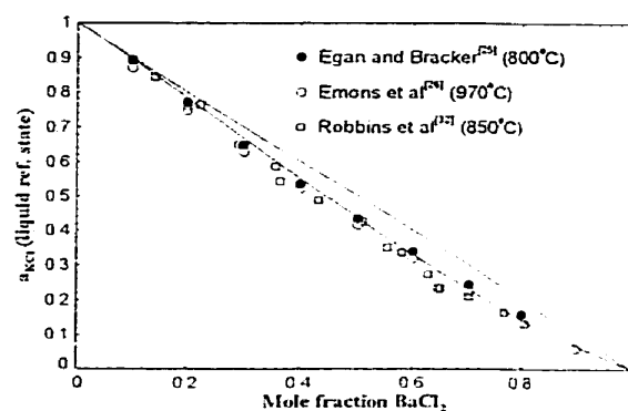
Fig. 11 – KCl-BaCl 2 system : calculated activity of KCl in the liquid at 800°C (liquid ref. state).
