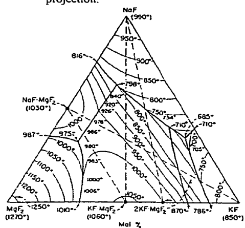
Fig. 11 - NaF-KF-MgF 2 system : experimental liquidus projection of Bergman and Dergunov [14] .
