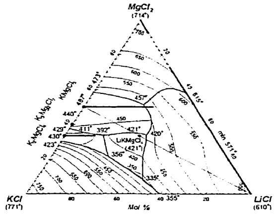
Fig. 21 - LiCl-KCl-MgCl 2 system : calculated liquidus projection.
