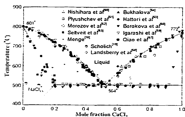
Fig. 34 - \text{NaCl-CaCl}_2 system : calculated phase diagram.
