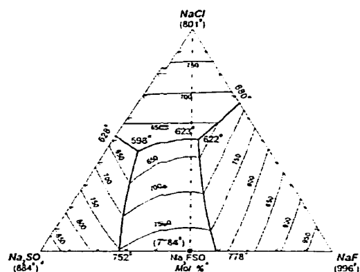
Fig. 3 - Calculated Na 2 Cl 2 -Na 2 F 2 -Na 2 SO 4 liquidus projection
