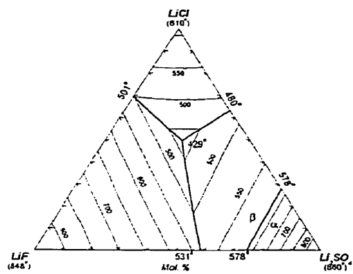
Fig. 1 - Calculated liquidus projection of the LiCl-LiF-Li 2 SO 4 system (predicted).
