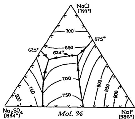
Fig. 2 - Measured NaCl-NaF-Na 2 SO 4 liquidus projection of Wolters [13] projection.
