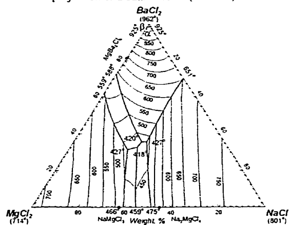
Fig. 30 - \text{NaCl} - \text{MgCl}_2 - \text{BaCl}_2 system : calculated liquidus projection.
