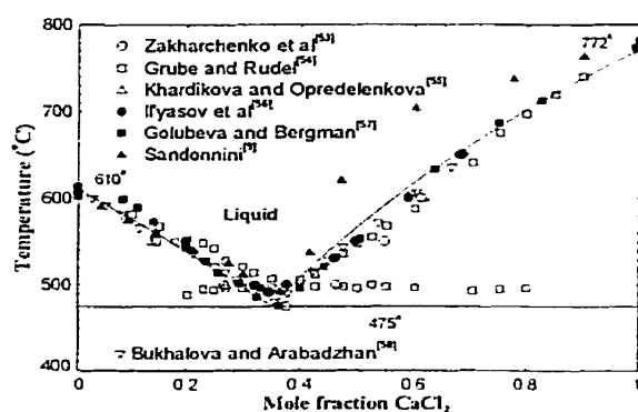
Fig. 31 - \text{LiCl-CaCl}_2 system : calculated phase diagram.
