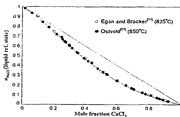
Fig. 35 - \text{NaCl-CaCl}_2 system : calculated activity of \text{NaCl} in the liquid at 825°C (liquid ref. state).
