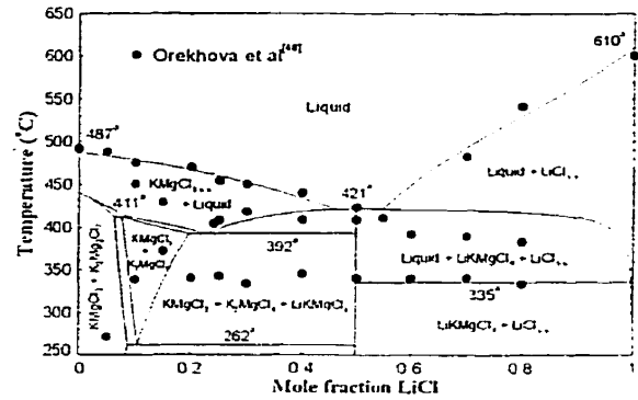
Fig. 22 - LiCl-KCl-MgCl 2 system : calculated KMgCl 3 -LiCl join
