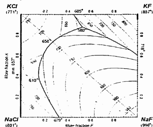
Fig. 11 - Na,K/F,Cl system : calculated liquidus projection.
