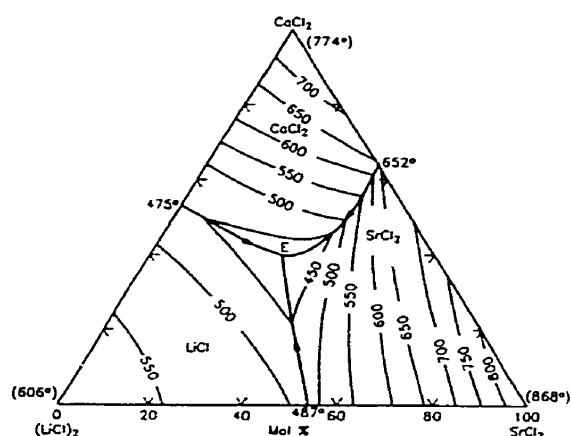
Fig. 28 – Li 2 Cl 2 -CaCl 2 -SrCl 2 system : experimental liquidus projection of Khardikova and Opredelenkova [28] .
