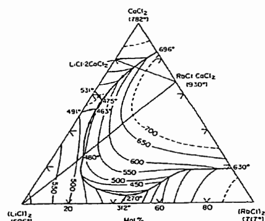
Fig. 47 - (\text{LiCl})_2 - (\text{RbCl})_2 - \text{CaCl}_2 system : experimental liquidus projection of Il'yasov et al. [56].
