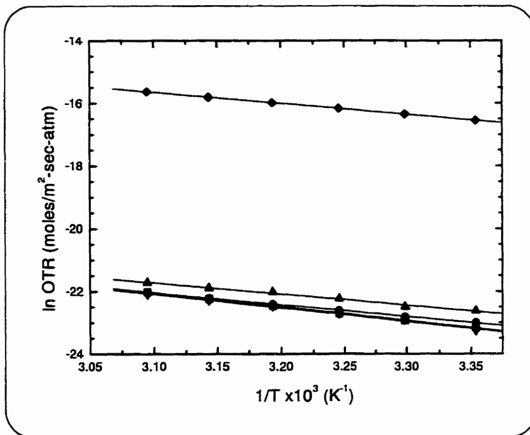
Figure 7.10: Arrhenius plot for OTR through PET (♦), \text{SiO}_2/\text{PET} (▲), \text{SiN}/\text{PET} (■), \text{SiO}_2/\text{PET}/\text{SiO}_2 (▼) and \text{SiN}/\text{PET}/\text{SiN} (●) film systems, in the 25 °C - 50 °C temperature range.
