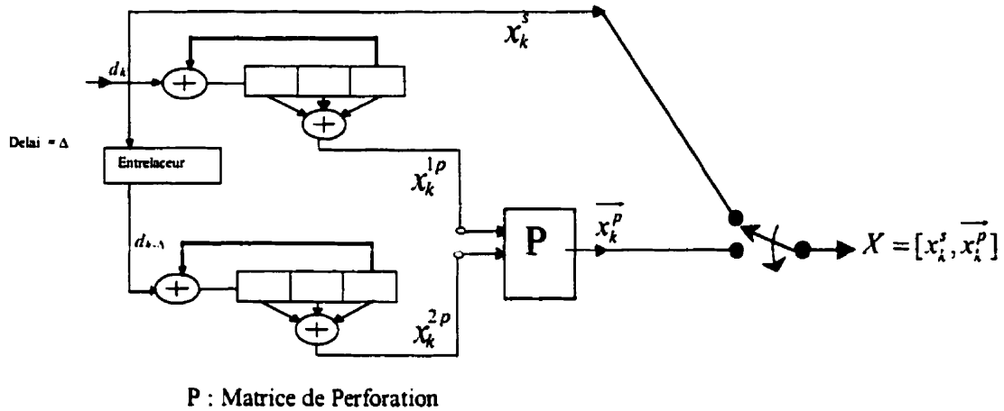
Figure 2.7: Codeur Turbo
