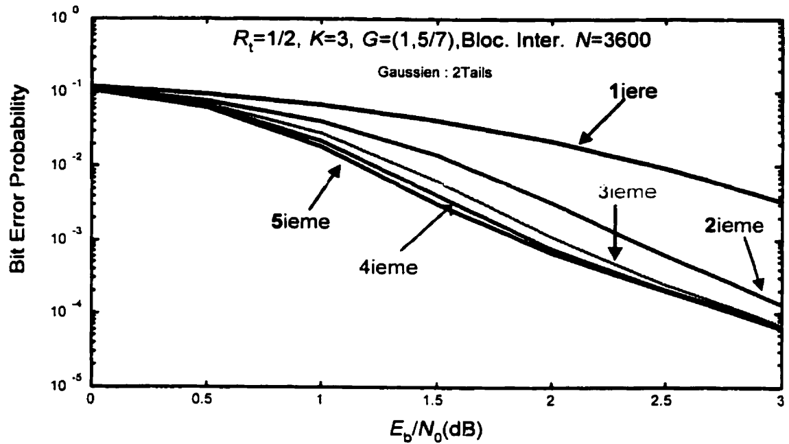
Figure 4.10: BER, K = 3 , R_t = 1/2 , N = 3600 , Entrel. Bloc, Canal AWGN, Terminaison : 2Tails.
