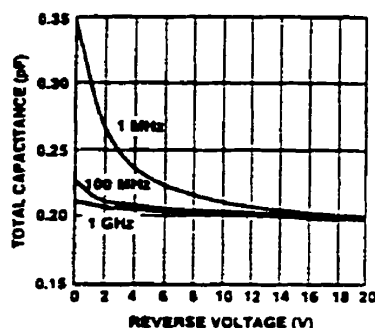
Figure 2. RF Capacitance vs. Reverse Bias. HSMP-386B/C/E/F Series.
