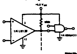
Driving CMOS
