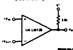
Basic Comparator
