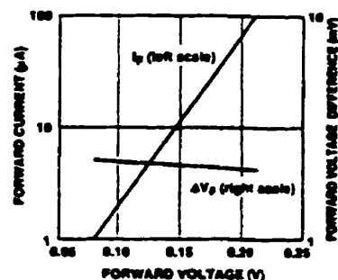
Figure 3. Typical Forward Voltage Match, HSMS-2860 Pairs.
