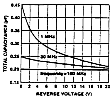
Figure 1. RF Capacitance vs. Reverse Bias. HSMP-381B/C/E/F Series.
