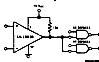
Driving TTL
