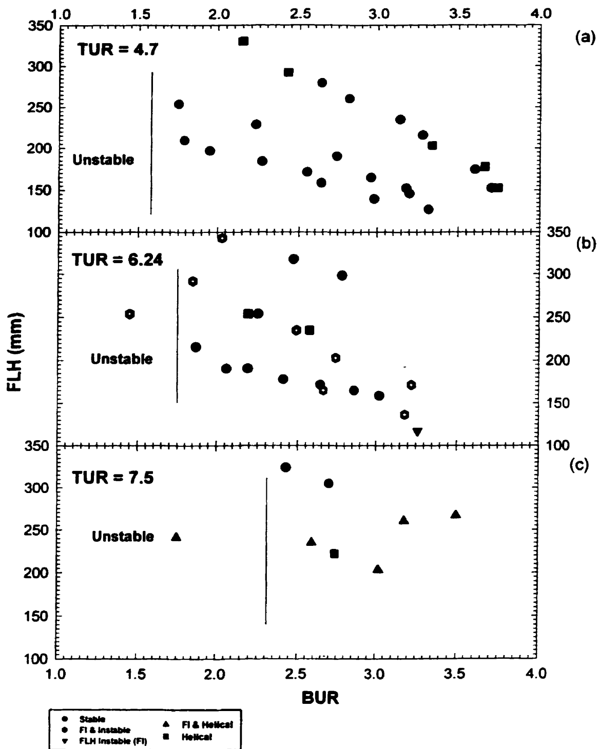
Figure 4.18. Bubble stability behavior of mPE under the extrusion temperature = 200°C, Flow rate = 5.4 Kg/h (a) TUR = 4.7, (b) TUR = 6.24, (c) TUR = 7.5.
