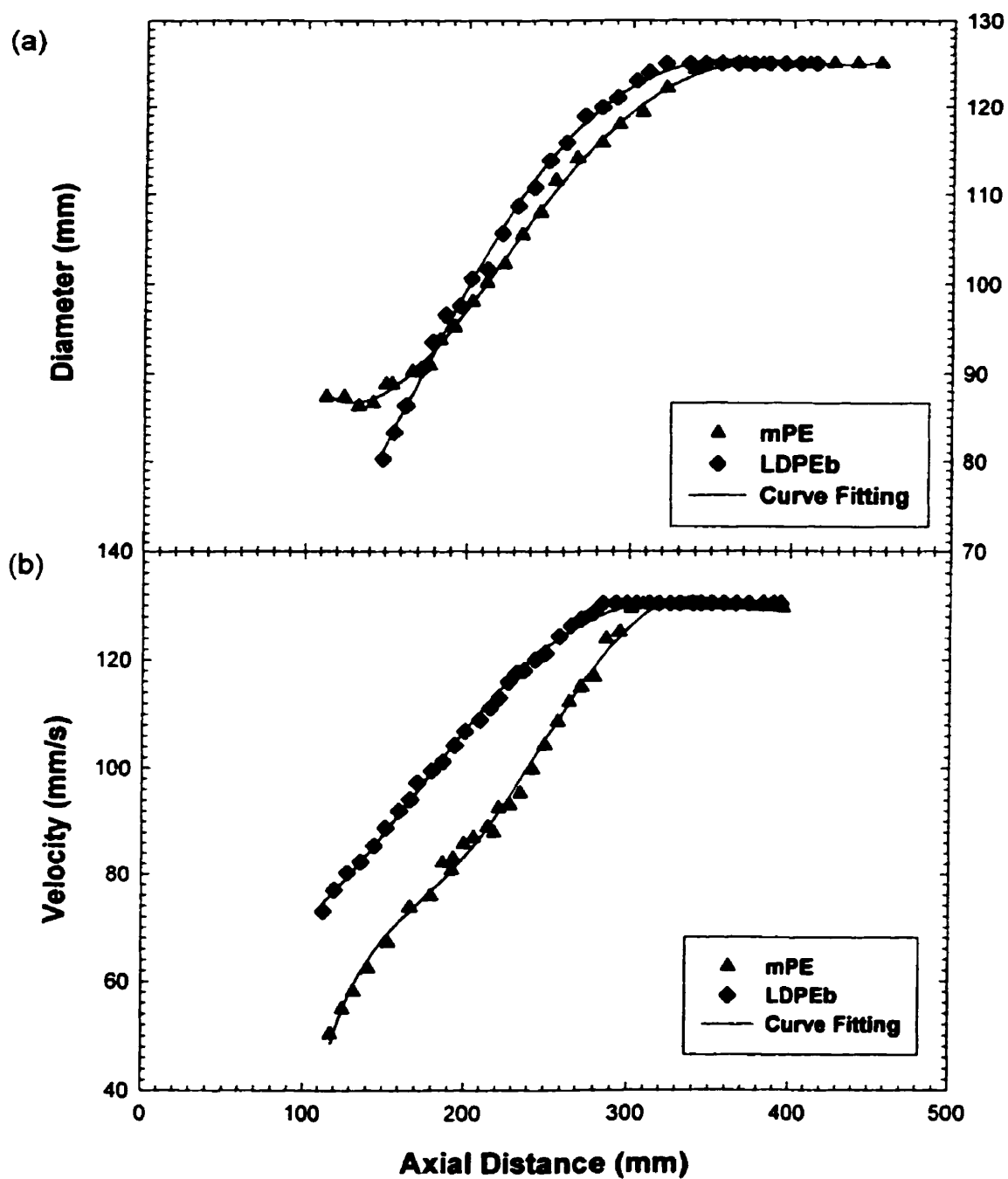
Figure 4. 13. Bubble diameter (a), velocity (b), and thickness (c) profiles along the axial distance for mPE and LDPEb. The film blowing conditions are the same as in Figure 4.10.
