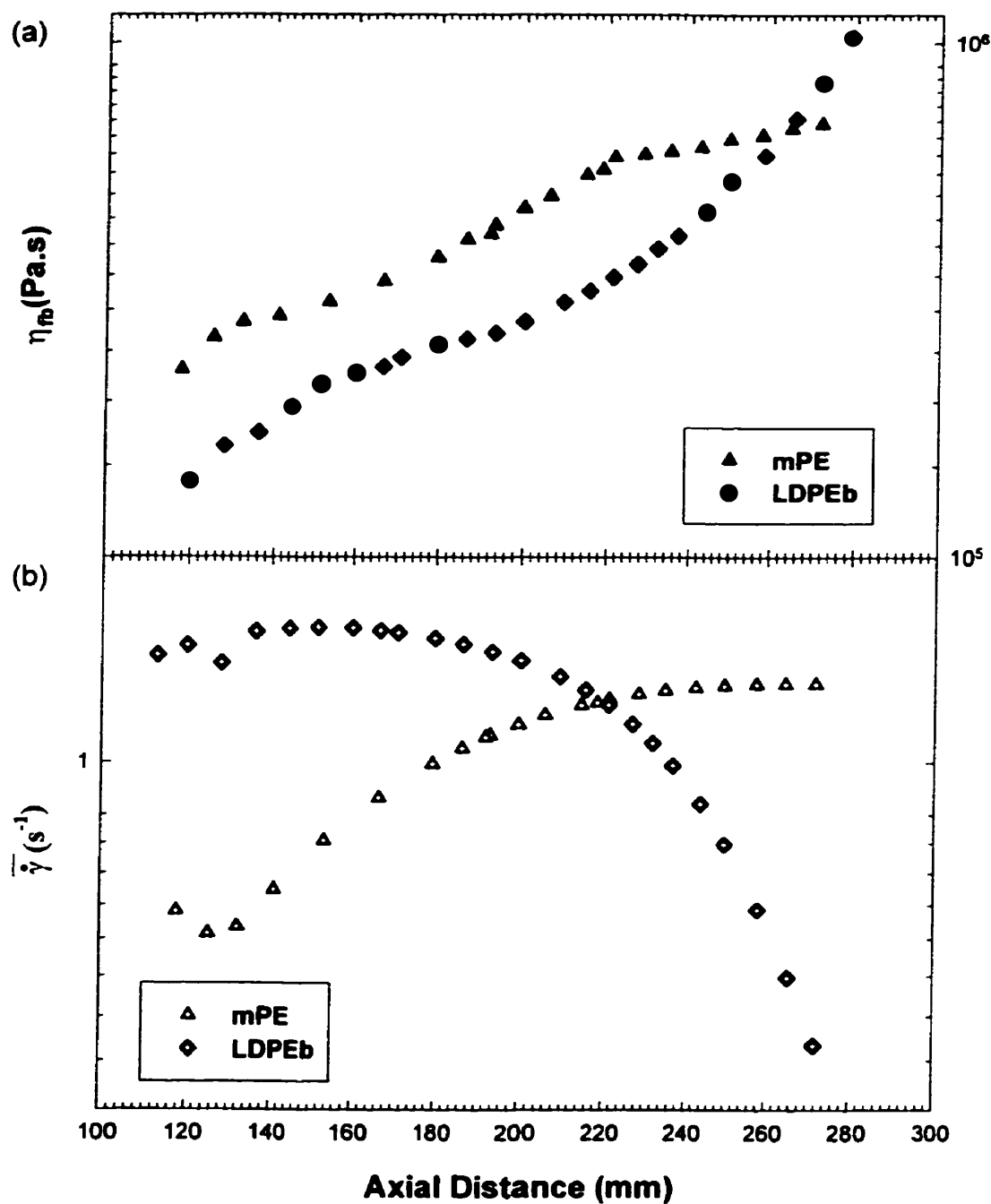
Figure 4.17. Apparent biaxial elongational viscosity (a) and the effective deformation rate (b) profiles along the axial distance for mPE and LDPEb. The film blowing conditions are the same as in Figure 4.10.
