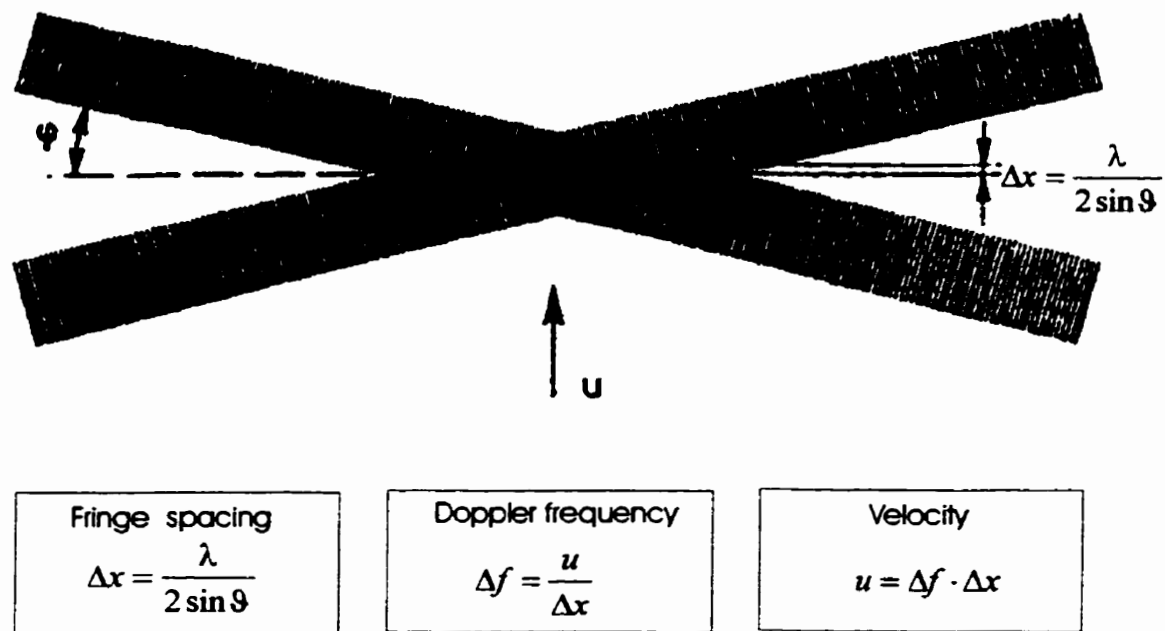
Figure 3. 3. Interference pattern model in the Laser Doppler Velocimetry (LDV) (adopted from Michaeli and Schmitz, 1995).
