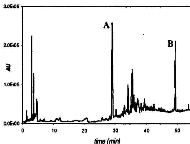
Figure 2.12 RP-HPLC chromatogram of control catheters ; (A) N,N'-bis ethylene stearamide; (B) antioxidant Irganox 1076 (Analysis on a C8 LiChrospher60 column (5 \mu m), 250x4 mm i.d. Phase A : 100/125 ACN/H 2 O, Phase B: THF - Gradient:0-15min,100 % A ; 15-60 min, 100% A to 100% B - Flow rate : 1 ml/min ; UV detector \lambda =280 nm)
