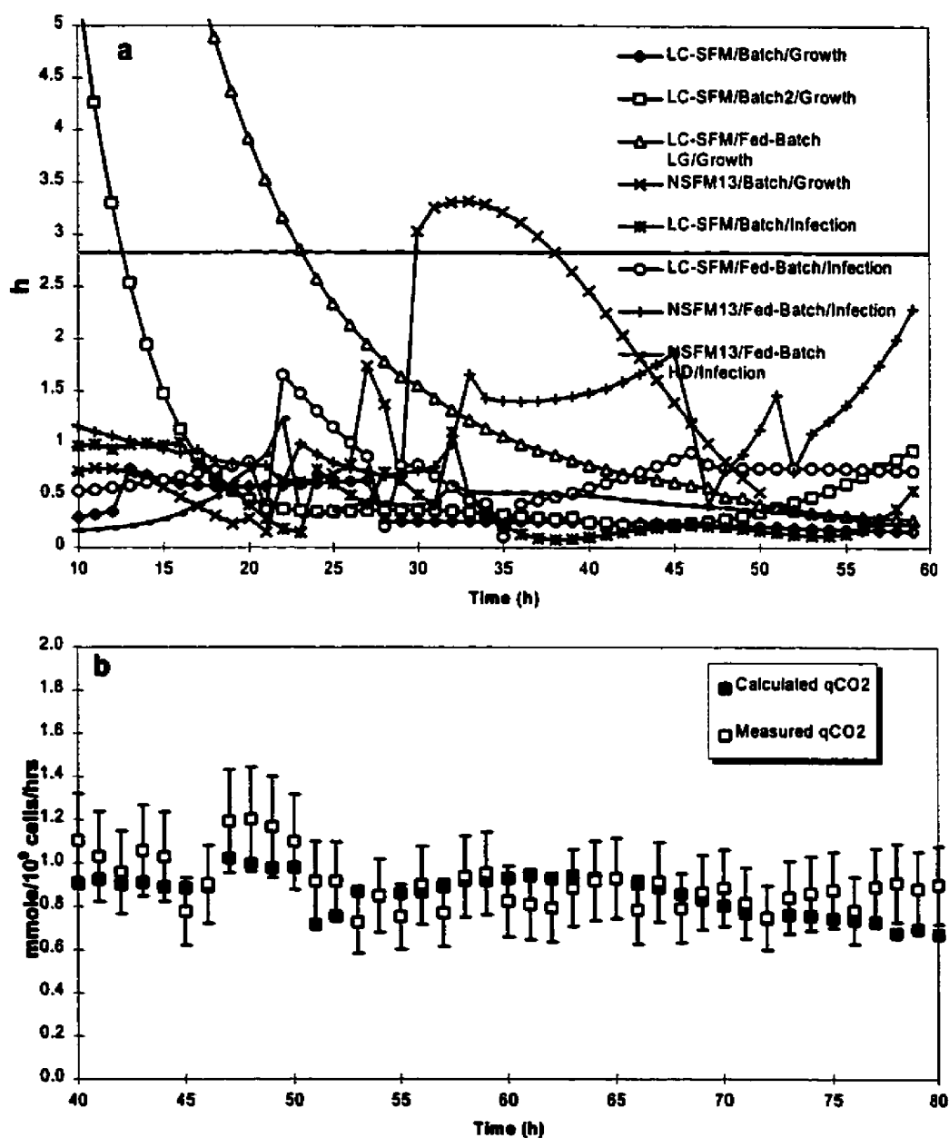
Figure 5.4 a) criteria h b) Calculated \text{CO}_2 versus measured \text{CO}_2 with the model
