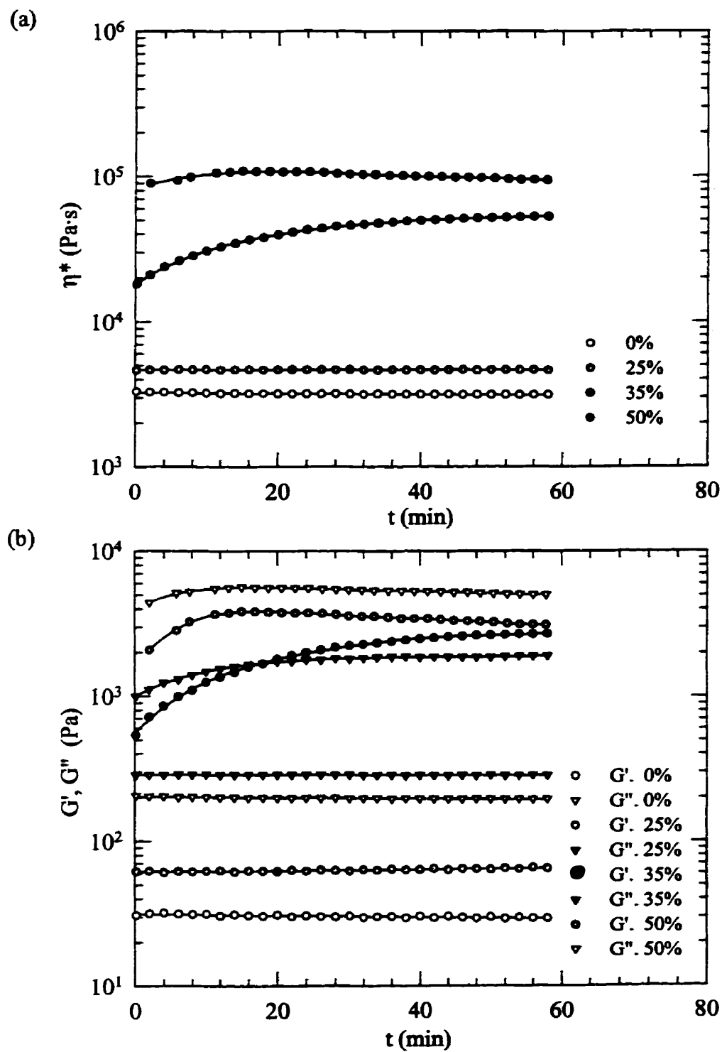
Figure 5.1: Variations of rheological properties with time measured at T=200^{\circ}\text{C} and 0.01 Hz for PP with \text{CaCO}_3 (UF) (dps1): (a) \eta^* , (b) G' & G''
