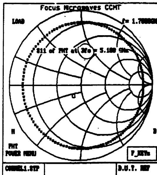
Harmonic Impedances of 1.6 and 1.7GHz
