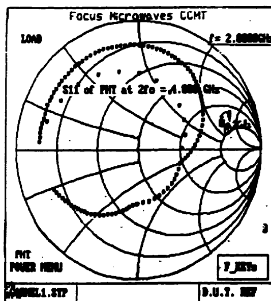
Harmonic Impedances of 1.9 and 2.0GHz
