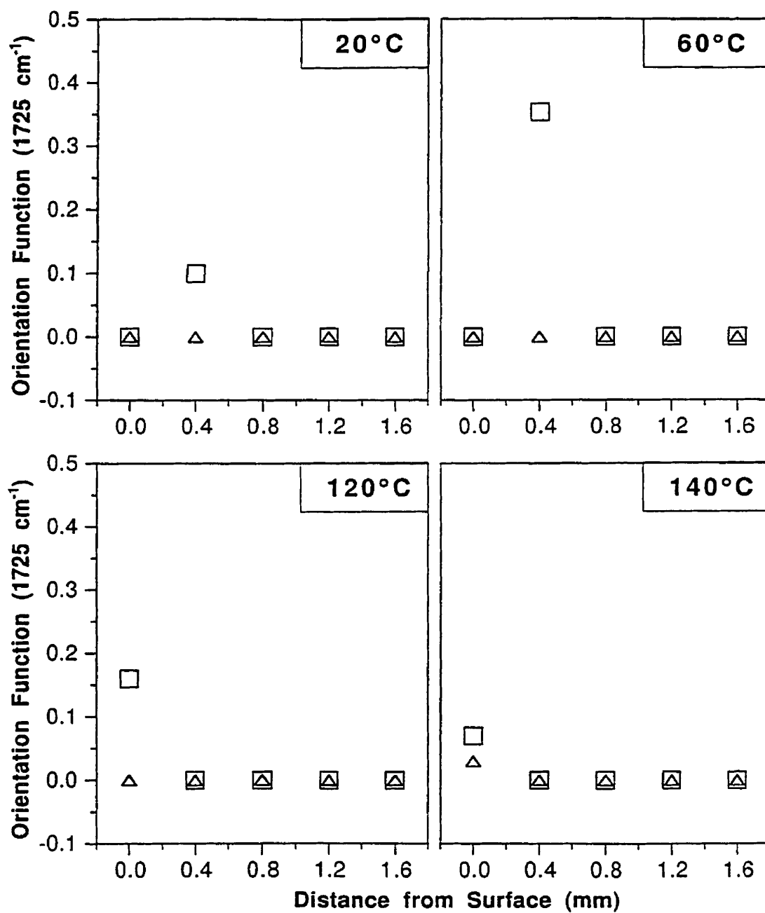
Figure 4.15. Variation of the molecular orientation function in the thickness direction for different mold temperatures, near the gate ( \square ) and far from the gate ( \Delta ), based on the dichroism of the peak at 1725\text{ cm}^{-1} .
