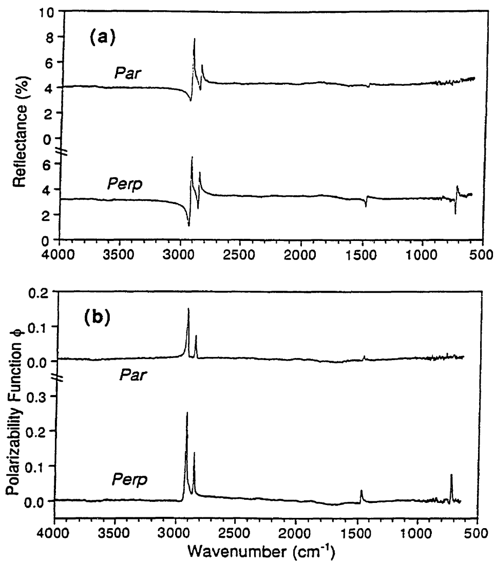
Figure 3.8 - Reflectance spectra (a) and corresponding polarizability spectra (b) measured at the surface of the oriented HDPE sample after milling and polishing with water as cooling medium
