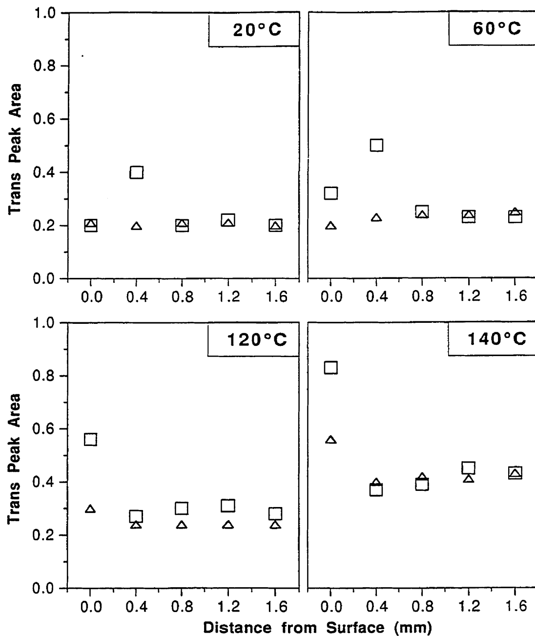
Figure 4.13. Variation of the glycol trans peak area in the thickness direction for different mold temperatures, near the gate ( \square ) and far from the gate ( \Delta ).
