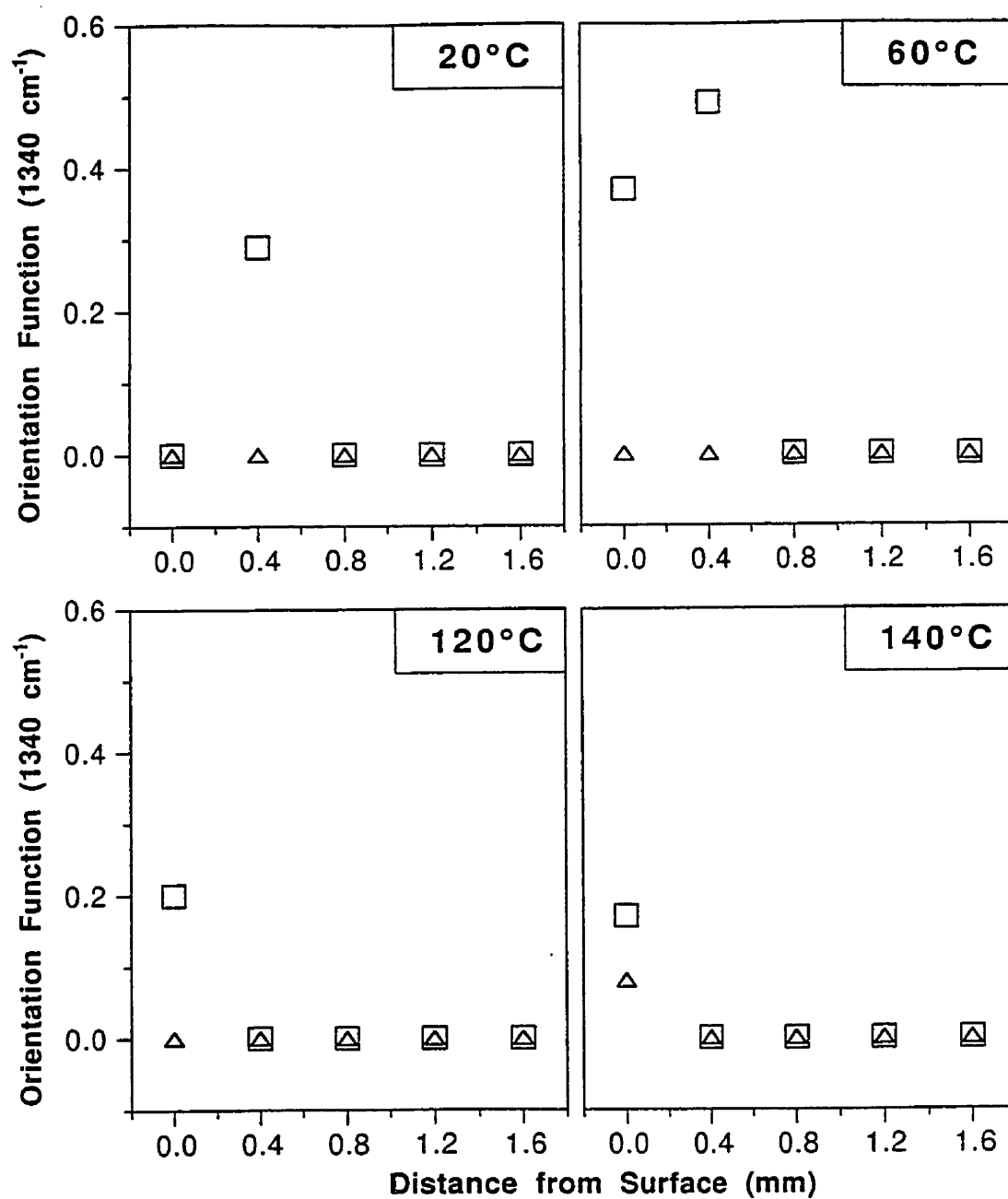
Figure 4.14. Variation of the molecular orientation function in the thickness direction for different mold temperatures, near the gate ( \square ) and far from the gate ( \Delta ), based on the dichroism of the peak at 1340\text{ cm}^{-1} .
