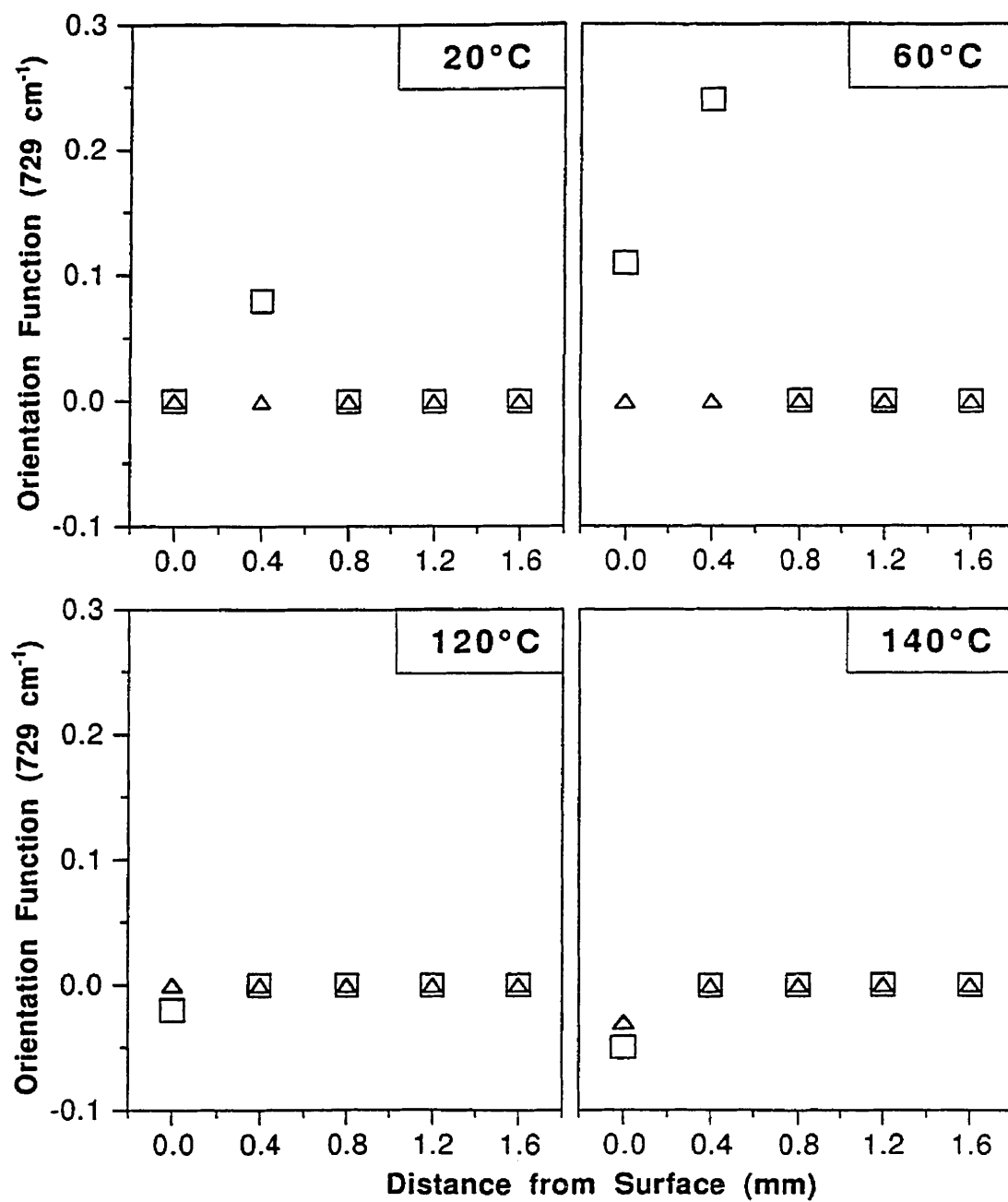
Figure 4.16. Variation of the molecular orientation function in the thickness direction for different mold temperatures, near the gate (□) and far from the gate (△), based on the dichroism of the peak at 729 cm -1 .
