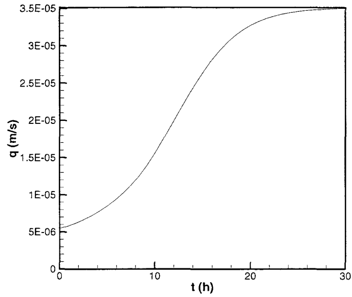
Figure 4.4: Time evolution of velocity
