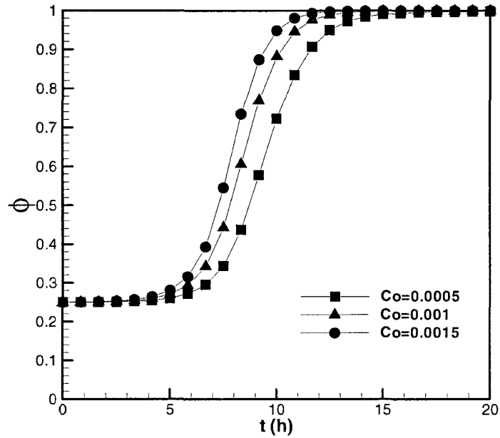
Figure 4.19: Time evolutions of porosity at x = L with different values of C_0
