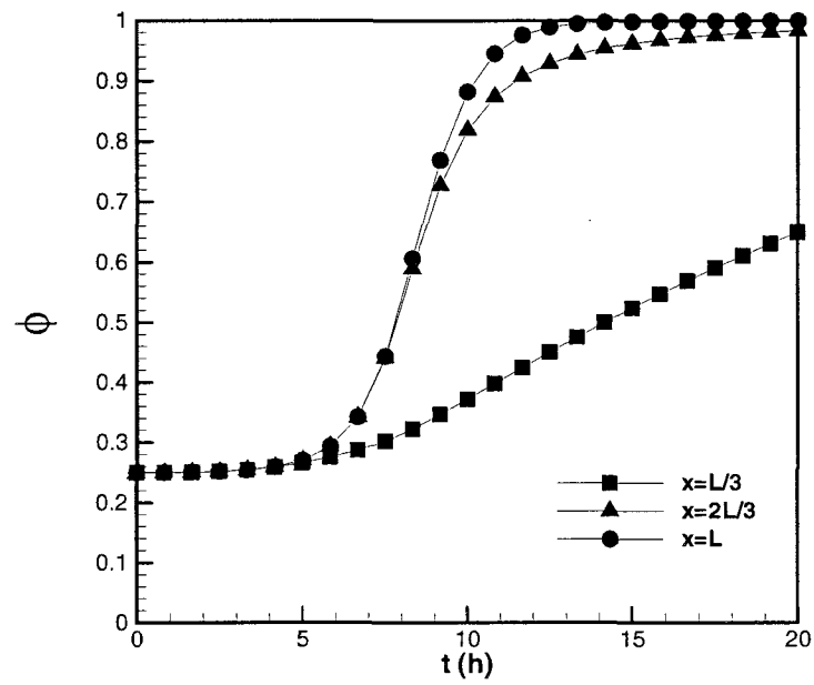
Figure 4.11: Time evolution of porosity
