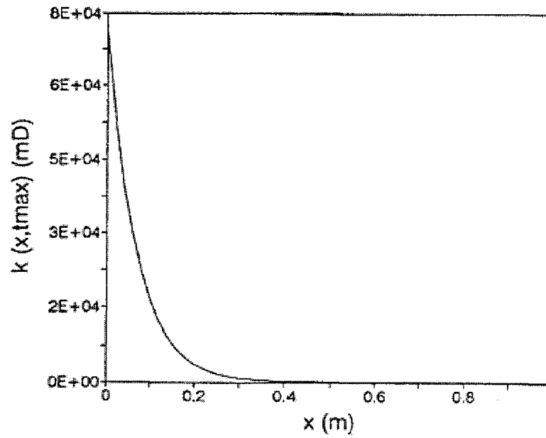
Figure 2.13: Spatial profile of permeability at 10^4 sec
