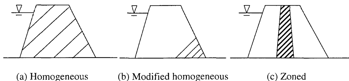
Figure 1.1: Types of earth-fill dams
