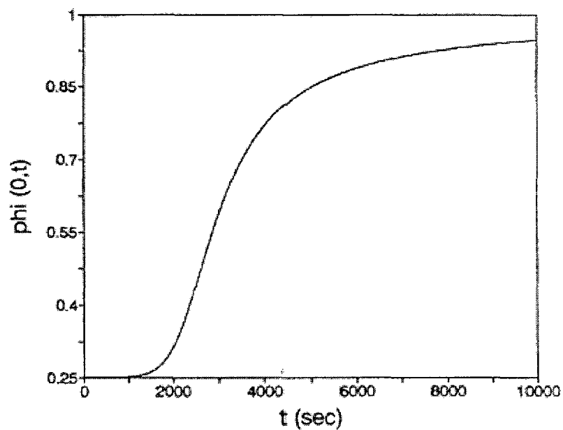
Figure 2.10: Time evolution of porosity at exit point
