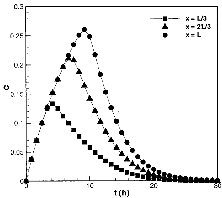
Figure 4.2: Time evolution of concentration
