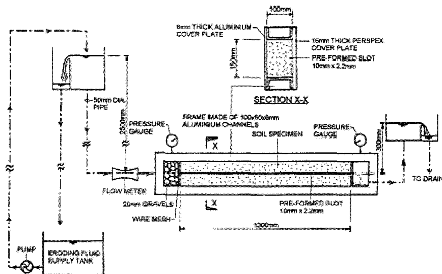
Figure 2.3: Schematic diagram of slot erosion test assembly
