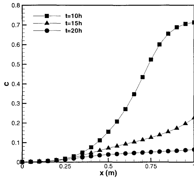
Figure 4.13: Spatial profiles of concentration at t = 10h, 15h and 20h
