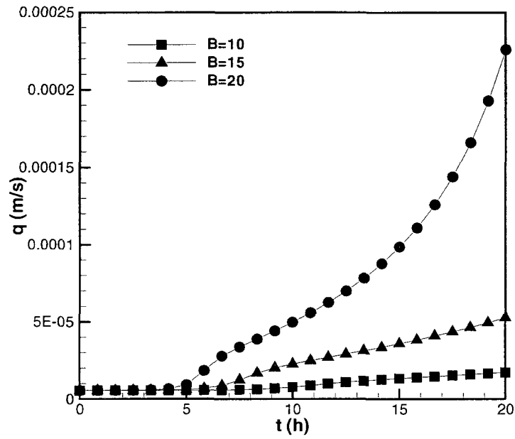
Figure 4.17: Time evolution of velocity with different values of B
