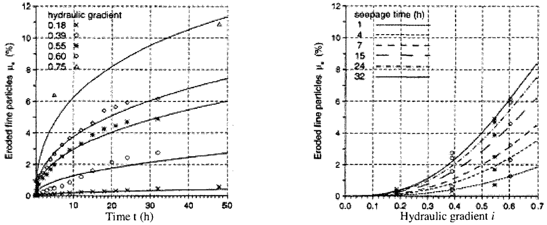
Figure 2.5: Variations in the percentage by weight of eroded fine particles with time (left) and with hydraulic gradient (right), from laboratory tests (dots) and from their analytical expression, eq. 2.6 (solid lines)
