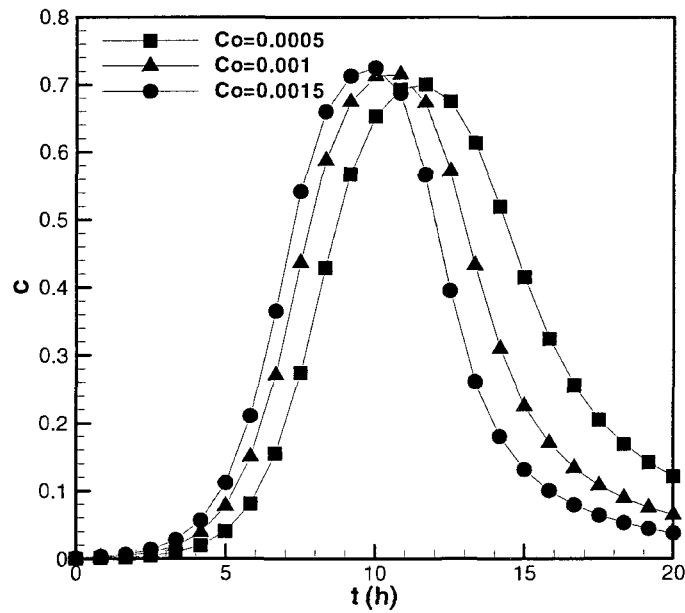
Figure 4.18: Time evolution of concentration at x = L with different values of C_0
