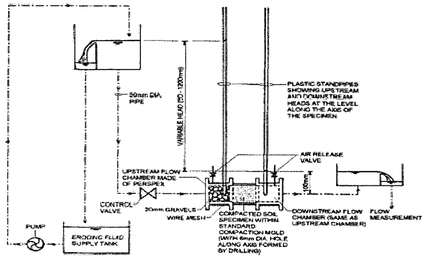
Figure 2.2: Schematic diagram of hole erosion test assembly
