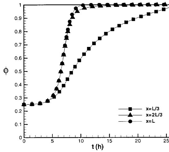
Figure 4.21: Time evolution of porosity with A = 0.01 , B = 15
