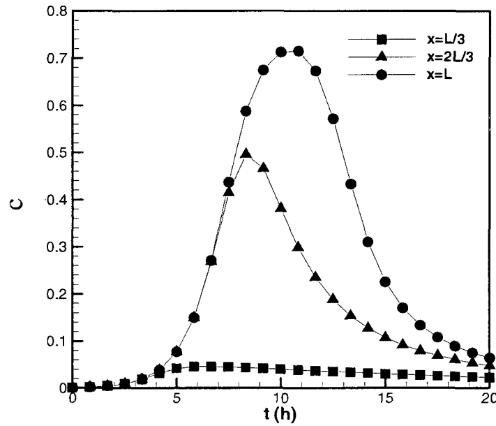
Figure 4.10: Time evolution of concentration
