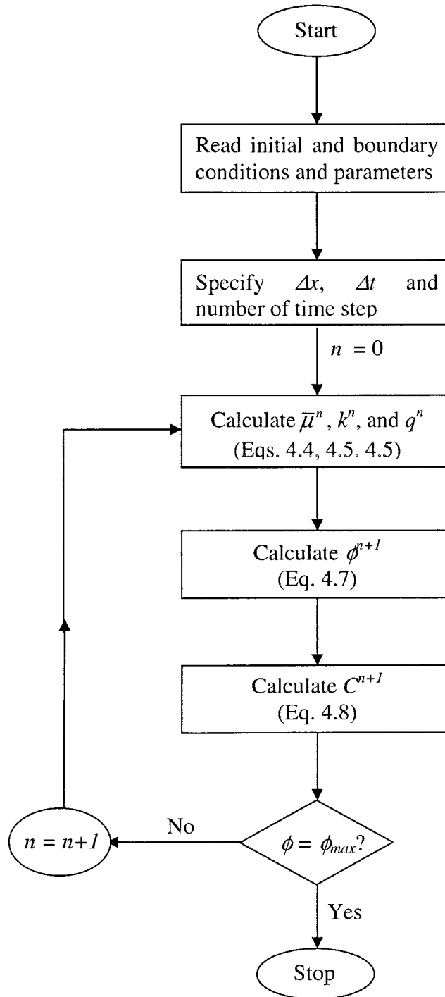
Figure 4.1: Flow chart of solution
