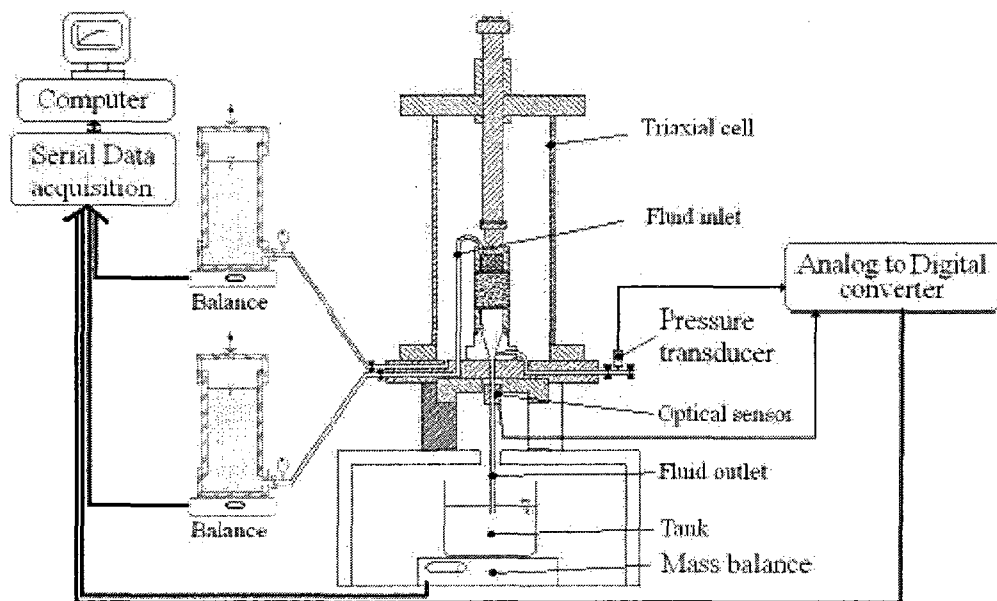
Figure 2.6: Schematic representation of the experimental triaxial cell.
