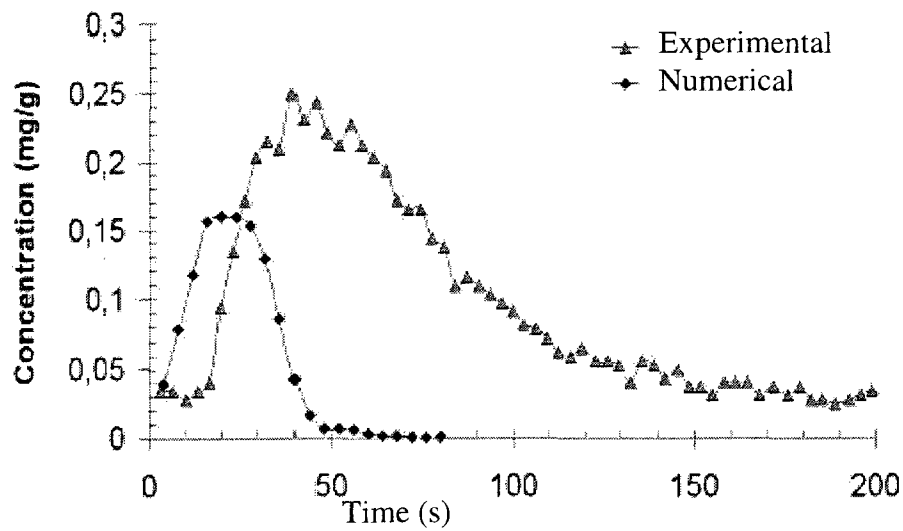
Figure 2.7: Time evolution of concentration of outflow
