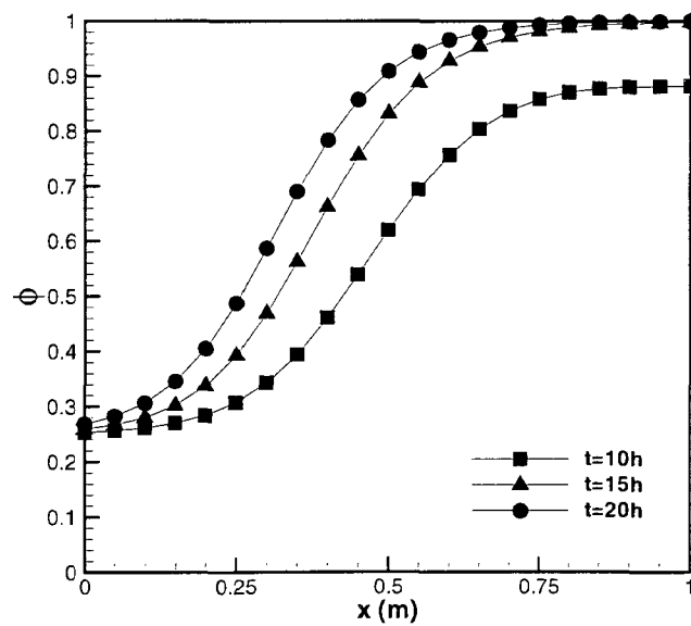
Figure 4.14: Spatial profiles of porosity at t = 10h, 15h and 20h
