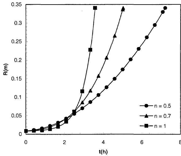
Figure 4.25: R vs t for various values of n
