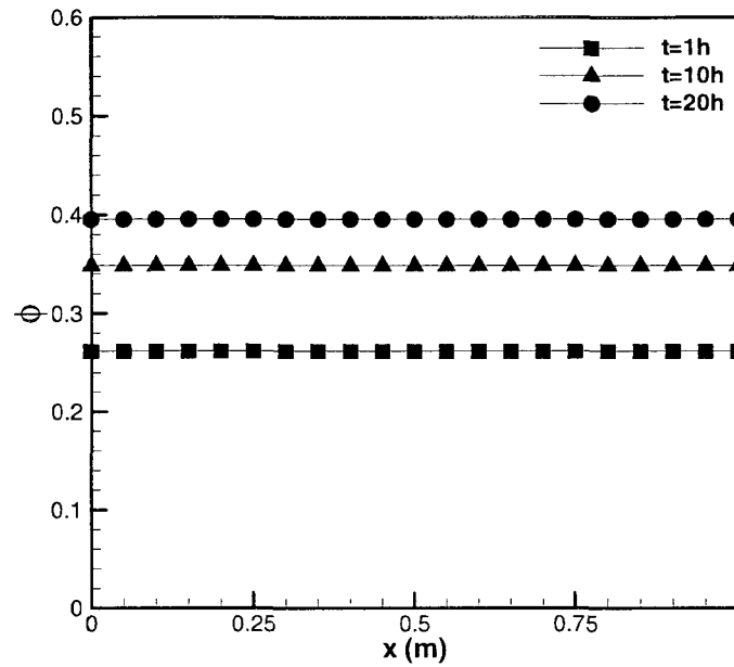
Figure 4.6: Spatial profiles of porosity at t = 10h, 15h and 20h
