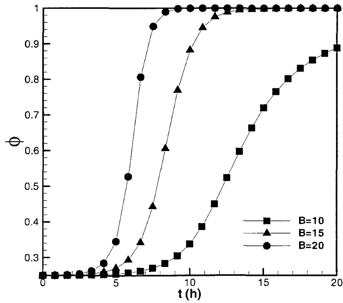
Figure 4.16: Time evolution of porosity at x = L with different values of B
