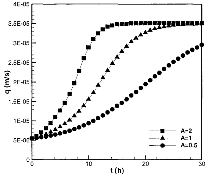
Figure 4.9: Time evolution of velocity with different values of A
