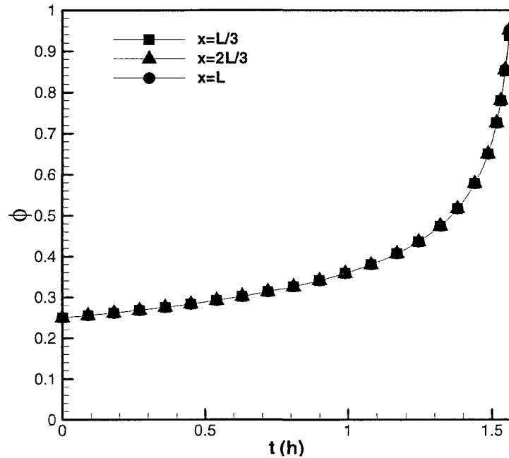
Figure 4.23: Time evolution of porosity with A = 1 , B = 15
