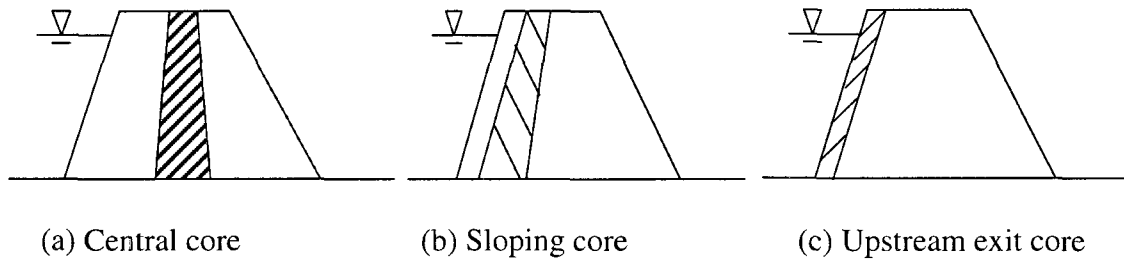
Figure 1.2: Types of rock-fill dams
