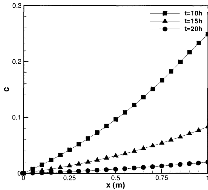
Figure 4.5: Spatial profiles of concentration at t = 10 h, 15h and 20h
