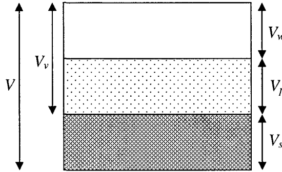
Figure 3.1: A volume element of a porous medium
