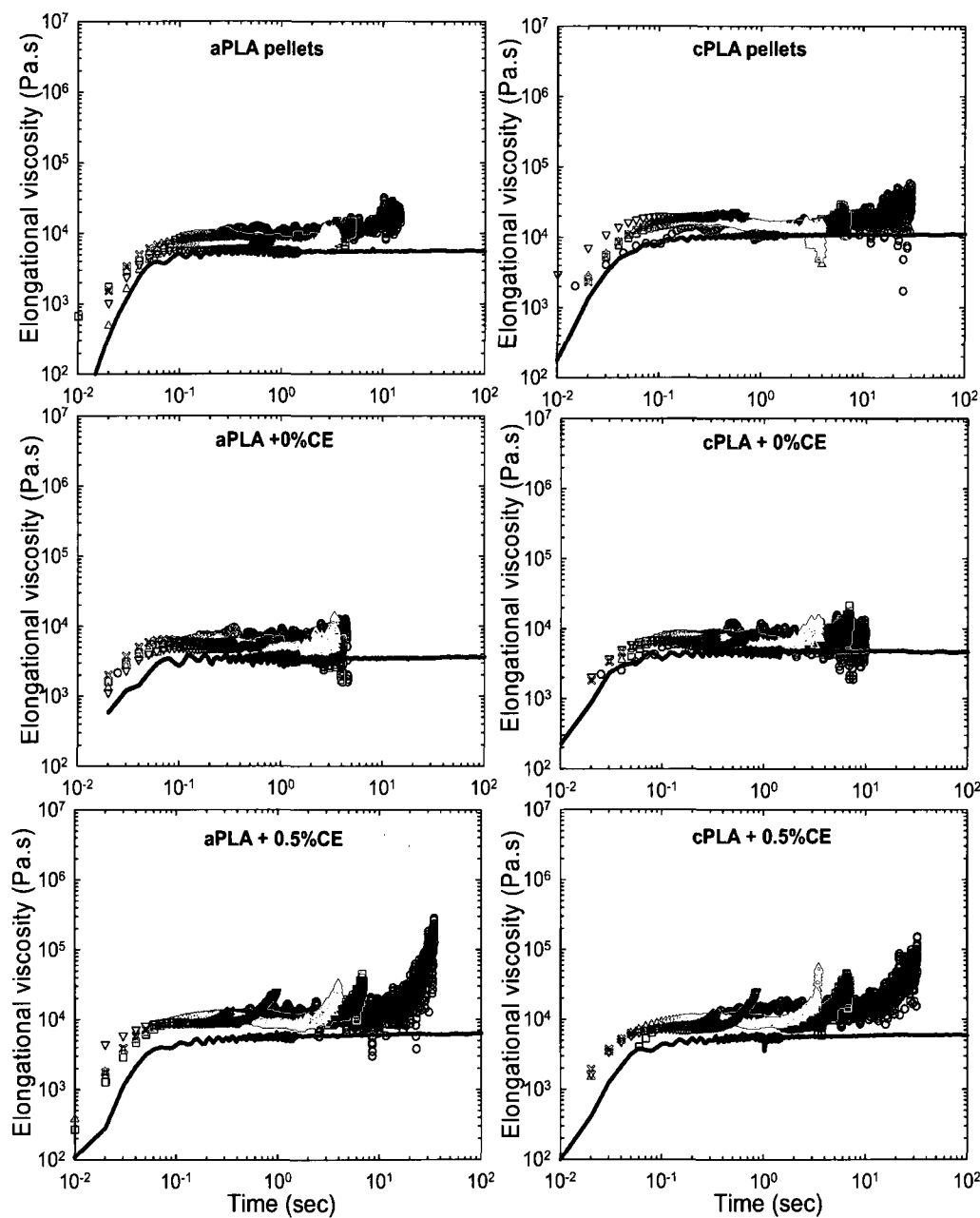
Figure 6.5 Elongational viscosity as a function of time of branched aPLA and cPLA with 0 - 2% chain extender. Hencky strain rates were: \circ - 0.1 \text{ s}^{-1} , \square - 0.5 \text{ s}^{-1} , \triangle - 1 \text{ s}^{-1} , \blacktriangledown - 5 \text{ s}^{-1} , \times - 10 \text{ s}^{-1} . The continuous curves represent the stress growth functions ( 3\eta^+ ) obtained in shear at \dot{\gamma} = 0.005 \text{ s}^{-1} .
