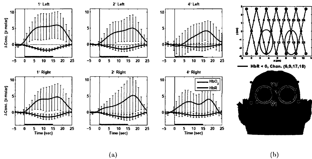
Figure 5.4 (a) Results of changes in \text{HbO}_2 (red) and \text{HbR} (blue) concentrations away from the inverted response channels during left (top) and right (bottom) stimulations for each eccentricity taken separately on source-detector channels {6, 9, 17, 18}. Clearly, each stimulation shows standard activation response ( p -values reported in Table 5.5). Gray shades indicate stimulation time. (b) Negative \text{HbR} regions (PBR) identified on the optodes configuration and the visual cortex.
