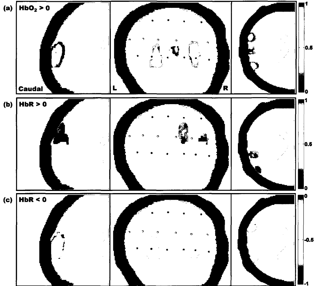
Figure 5.8 Reconstructed hemoglobin concentration changes using maximum intensity projection (MIP) overlaid on anatomical MRI (subject 4 in this case) in sagittal, coronal and axial views respectively. (a) Positive HbO_2 concentration changes. (b) Positive HbR concentration changes. (c) Negative HbR concentration changes. Remarks : all concentration changes come from real data ( 1^\circ left stimulus condition) with mean physiology removed. Units are arbitrary except for the sign. Red and blue dots on coronal views correspond to co-registered sources and detectors respectively. One can compare with temporal concentration changes from Fig. 5.6 and observe that reconstruction method correlates with spatial HbO_2 and HbR concentration changes.
