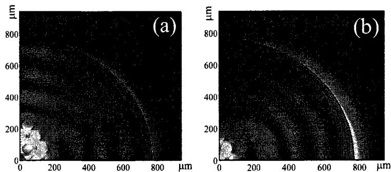
FIG. 6.4 – Longitudinal energy flux component distribution across the fiber crosssection for the core guided mode in the vicinity of a phase matching point with a plasmon. Plots (a) and (b) are calculated for the points (a) and (b) in Fig. 6.3a).
