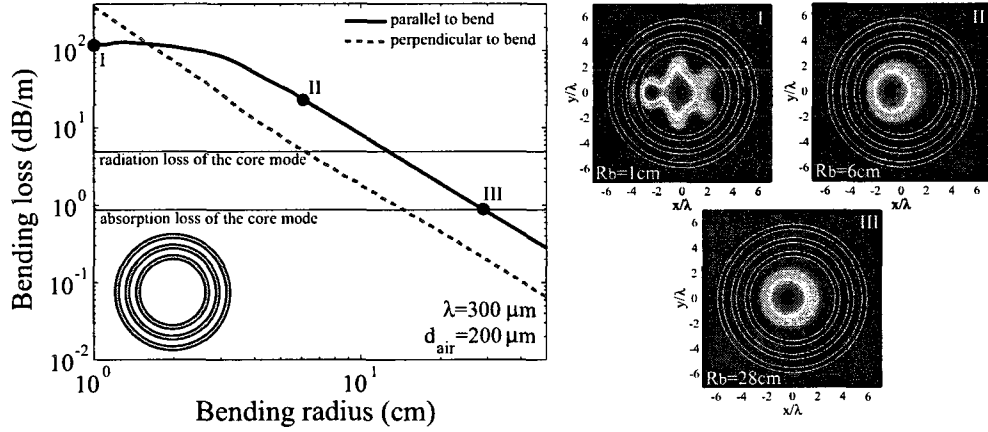
FIG. 4.7 – Bending losses of a porous Bragg fiber without bridges designed and operated at \lambda_c = 300 \mu\text{m} . Bending loss is strongly sensitive to the polarization of an HE_{11} mode, with the polarization in the plane of a bend being the lossiest. In the insets we show S_z flux distributions at the output of the 90^\circ bends of various radii.
