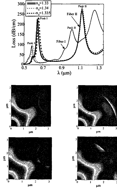
FIG. 2.3 – Calculated loss spectra of the core guided modes for two fiber designs. Loss spectra (solid lines) feature several attenuation peaks corresponding to the excitation of plasmonic modes on the surface of metallized channels filled with aqueous analyte n_a = 1.33 . By changing analyte refractive index (dotted lines) resonant attenuation peaks corresponding to the points of phase matching between the core guided and plasmon modes shift. In the insets, energy flux of a core guided mode is presented at various absorption peaks.
