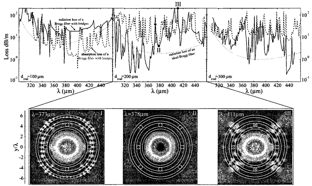
FIG. 4.6 – Radiation losses (solid lines) and absorption losses (dashed lines) of the hollow core Bragg fibers for various bridge sizes d_{rod} = [100, 200, 300] \mu m . For comparison, radiation loss of the equivalent Bragg fibers without rods are presented as dotted lines. Inset II shows S_z flux distribution in the fundamental core guided mode positioned at the minimum of the local bandgap at \lambda = 378 \mu m . Insets I and III show field distributions in the fundamental core mode at the wavelengths of coupling with different surface states.
