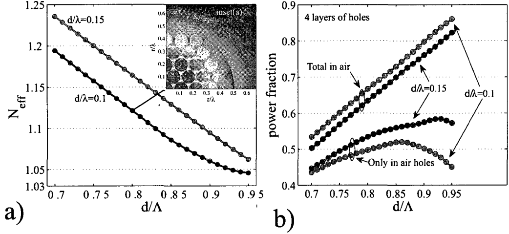
FIG. 4.2 – a) Effective refractive index of the fundamental core mode versus d/\Lambda for the two fiber designs having hole diameters of d/\lambda = [0.1, 0.15] . For the fiber with d/\lambda = 0.1 , distribution of the power flux in the waveguide cross-section S_z is shown for d/\Lambda = 0.8 in the inset (a). b) Fraction of modal power guided in the air as a function of d/\Lambda . The two upper curves show the total power fraction in the air (air plus cladding) while the two lower curves indicate the power fraction in the air holes only.
