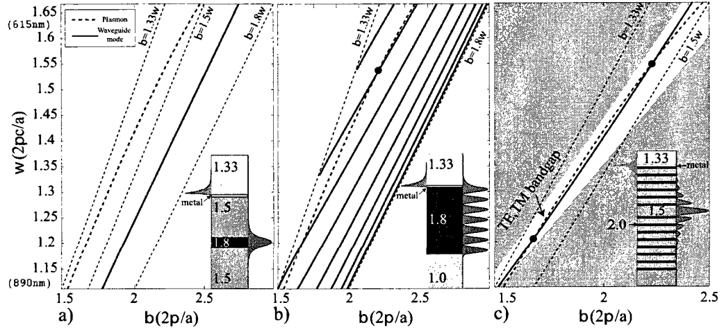
FIG. 3.1 – Band diagrams and schematics of various sensor implementations. a) Single mode waveguide-based sensor. Dispersion relations of a core guided mode (solid) and a plasmon (thick dashed). Inset - coupler schematic; |H_{||}|^2 of a plasmon (left) and a core mode (right). b) Multimode waveguide-based sensor. Dispersion relations of the core modes (solid) and a plasmon (thick dashed). Inset - coupler schematic; |H_{||}|^2 of a plasmon (left) and a high order mode (right) at the phase matching point (black circle). c) Planar photonic crystal waveguide-based sensor. Dispersion relation of a fundamental Gaussian-like leaky core mode (solid) and a plasmon (thick dashed). Inset - coupler schematic; |H_{||}| of a plasmon (left) and a core mode (right).
