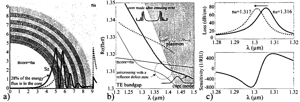
FIG. 3.5 – Analyte-filled large hollow core photonic crystal Bragg fiber-based SPR sensor. a) Schematic of a sensor. Analyte-filled hollow core is surrounded by a concentric photonic crystal reflector. Outside, the reflector is goldplated for plasmon excitation. Gold layer is bordered by aqueous analyte. Energy flux distribution across the fiber cross section is shown with a solid curve for the fundamental core mode, and with a dashed curve for the plasmonic mode. b) Band diagram of sensor modes. Dispersion relation of the fundamental core mode crossing over the analyte light line (thick solid curve), and plasmonic mode (dashed curve). TE bandgap of a periodic planar reflector is shown as a clear region, while gray regions correspond to the continuum of the bulk reflector states. c) Upper part: solid curve shows loss of the crossed-over core mode near the phase matching point with a plasmon at which modal loss peaks. Dashed line shows shift of the modal loss curve when refractive index of an analyte is varied. Lower part: dependence of the sensor amplitude sensitivity on wavelength.
