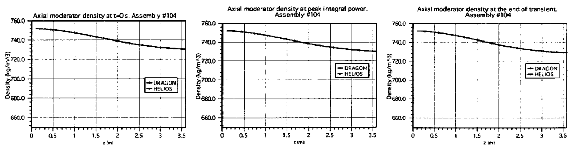
Figure III.18 UO 2 4.2% uncontrolled, burnup 37.5 GWd/t
