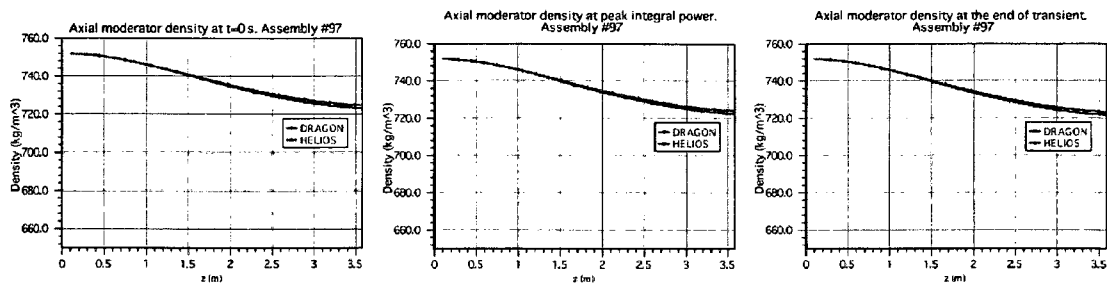
Figure III.16 UO 2 4.2% controlled, burnup 35 GWd/t
