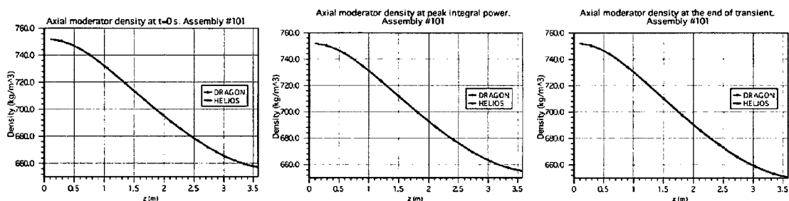
Figure III.17 UO 2 4.5% uncontrolled, burnup 37.5 GWd/t
