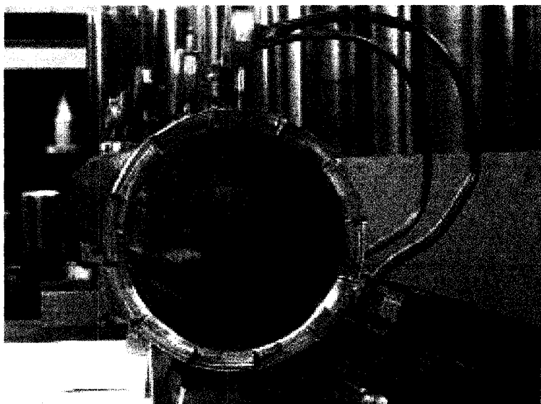
Figure 4.56: Flow formed Inconel 718 micro inch finish in the ID
