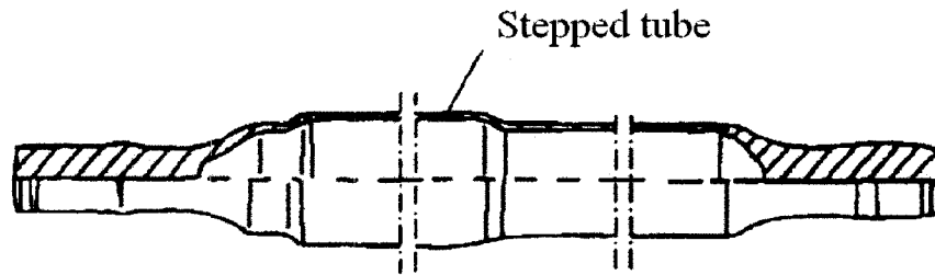
Figure 1.8: Both drive shafts ends welded to multi-stepped middle section (Thick/thin wall thickness). P. Amborn, H. Frielingsdorf, S.K. Ghosh and K. Greulich (1995) [2]
