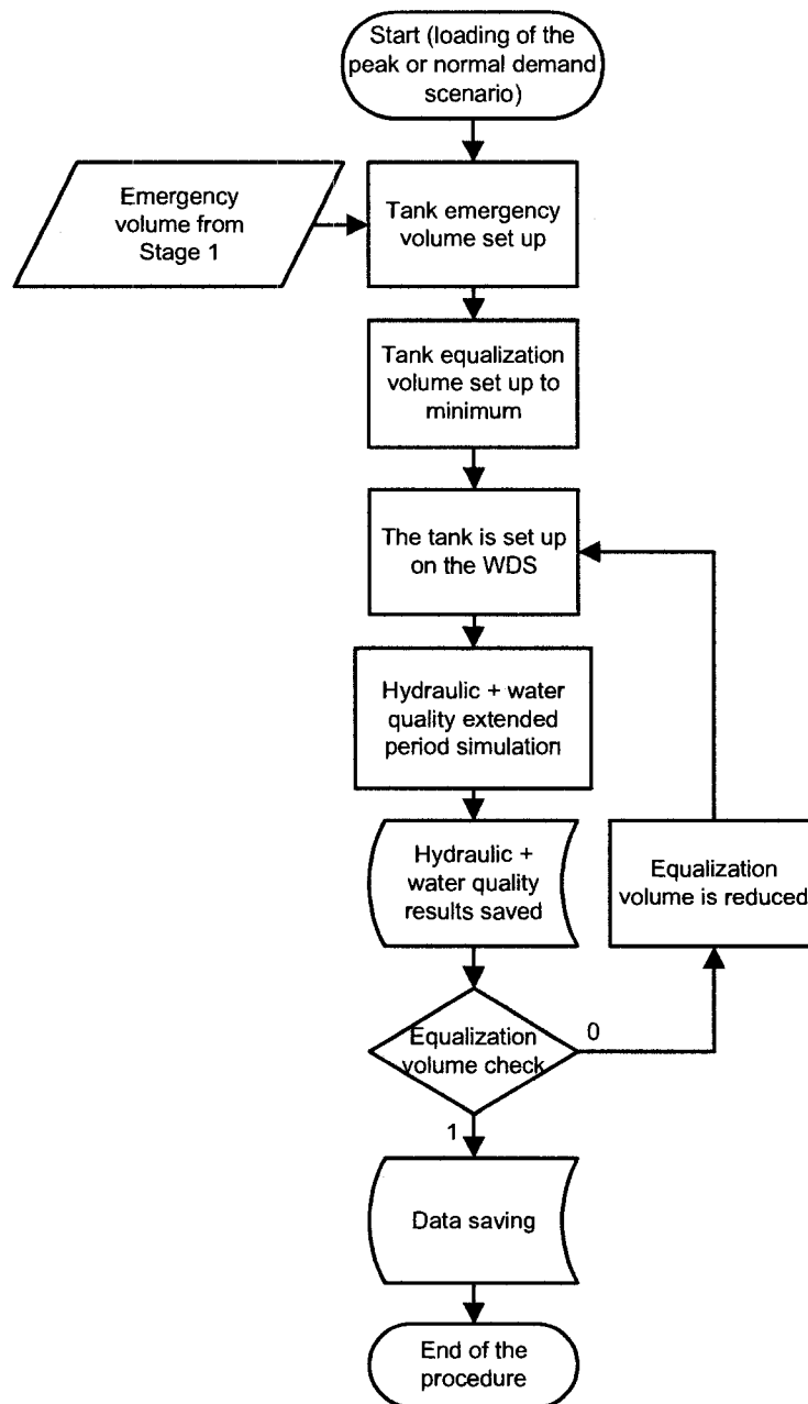
Figure 3.8 - Determination of the influence of the equalization volume for a ground tank
