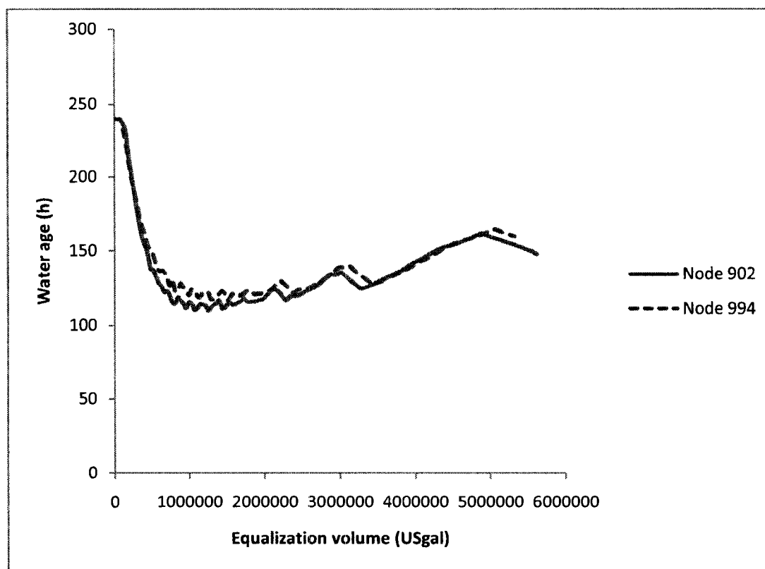
Figure 4.9 - Equalization volume vs. water age in the tank for both configurations (nodes 902 & 994)
