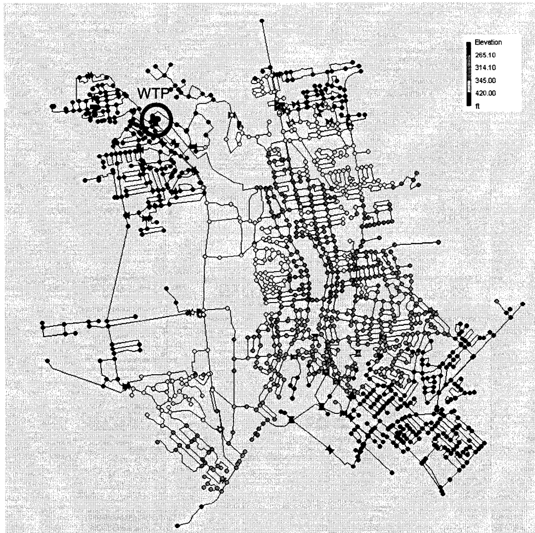
Figure 4.5 - Saint-Jérôme WDS layout and elevations
