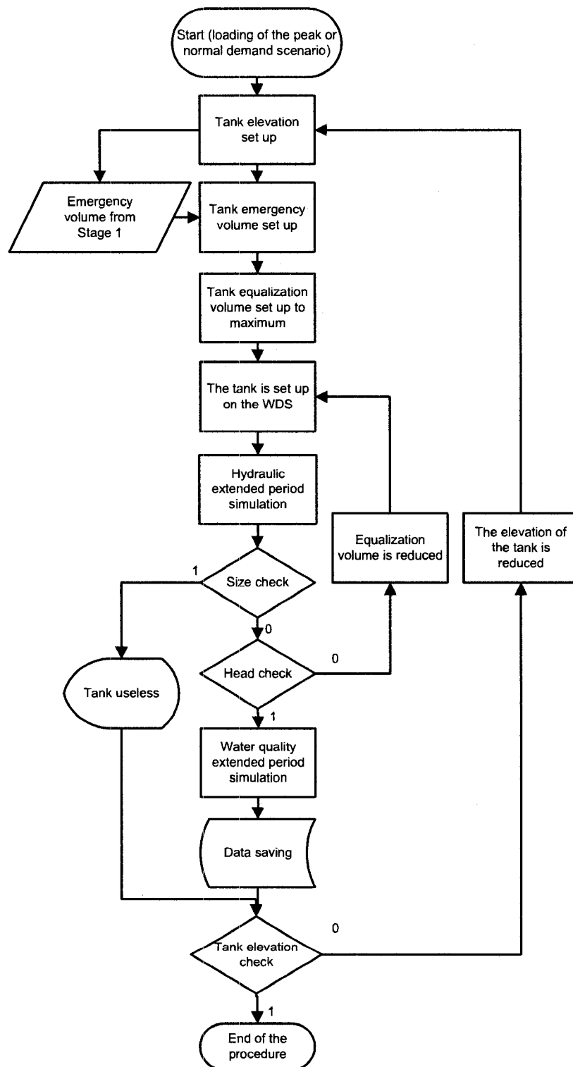
Figure 3.5 - Equalization volume determination for an elevated tank
