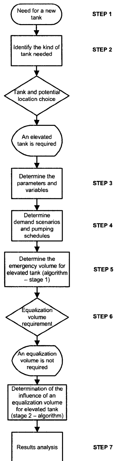
Figure 4.3 - Summary of the proposed methodology for sizing a storage tank
