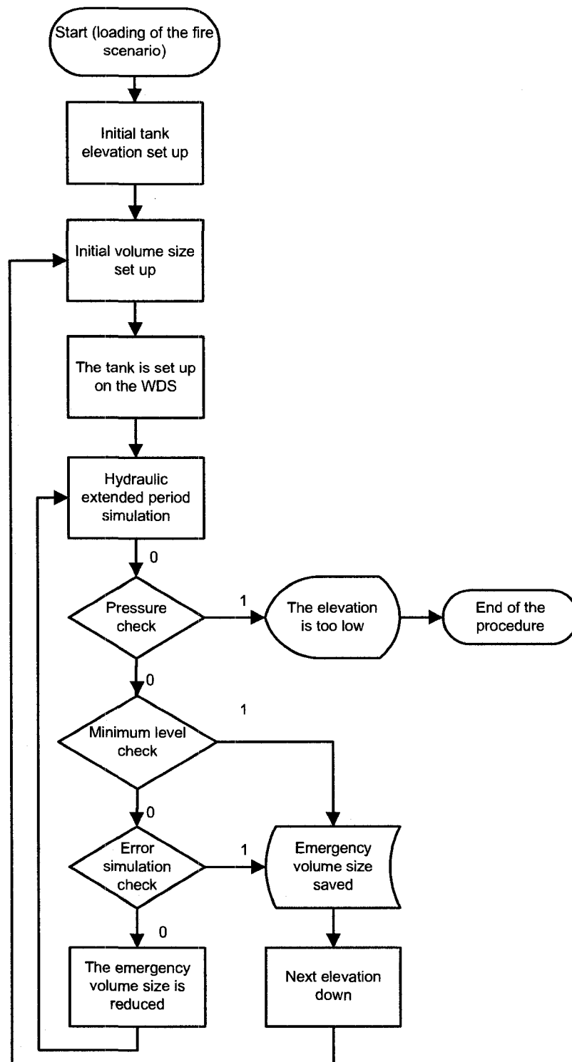
Figure 3.3 - Emergency volume determination for elevation tank
