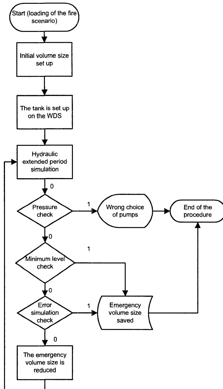
Figure 3.4 - Emergency volume determination for a ground tank
