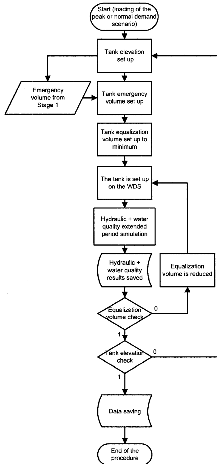
Figure 3.6 - Determination of the influence of the equalization volume for an elevated tank
