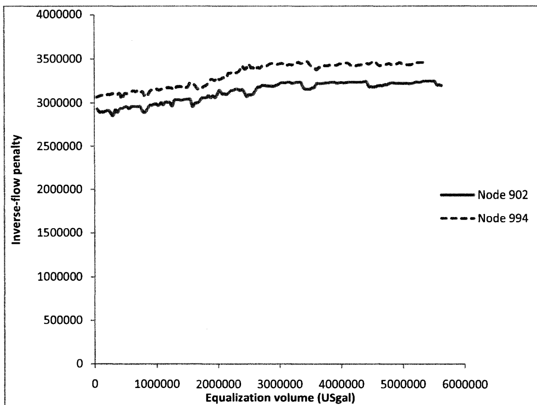
Figure 4.8 - Equalization volume vs. inverse-flow penalty in the tank for both configurations (nodes 902 & 994)
