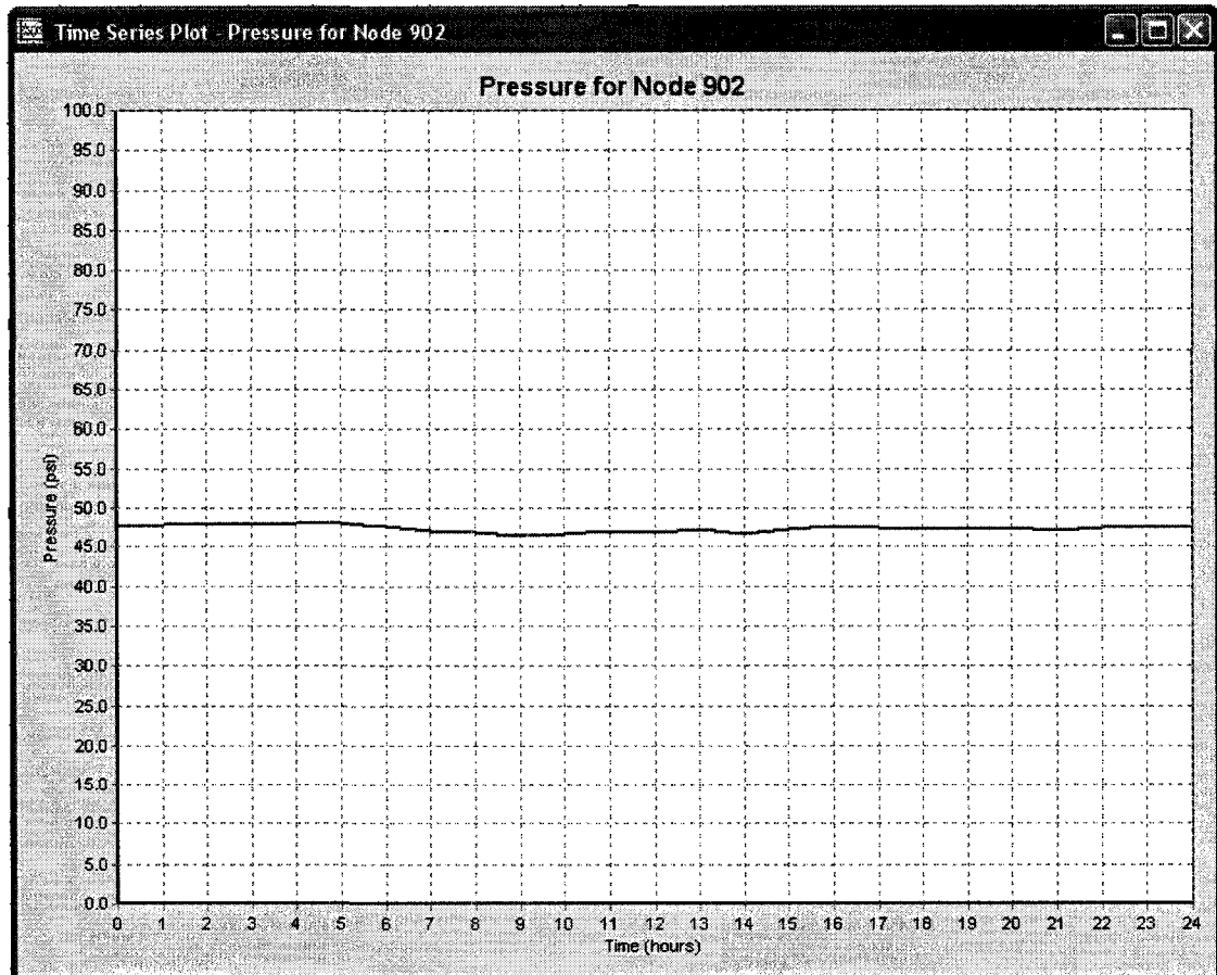
Figure 4.7 - Pressure variations at a potential tank location during normal flow condition simulation
