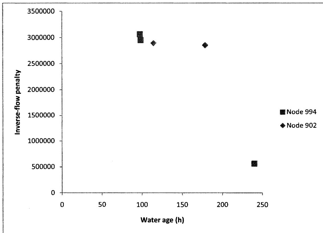
Figure 4.10 - Equalization volume vs. water age in the tank for both configurations (nodes 902 & 994)
