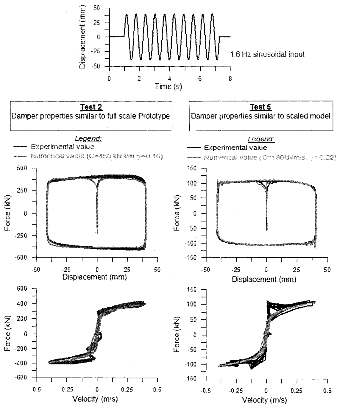
Figure 6.8: Input S3.3 – 1.6 Hz sinusoidal input of ten cycles.
