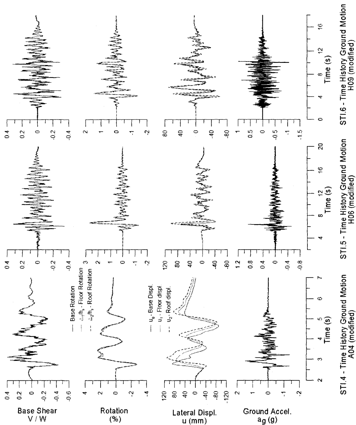
Figure 7.21: Test specimen response to the Vancouver ground motion inputs.
