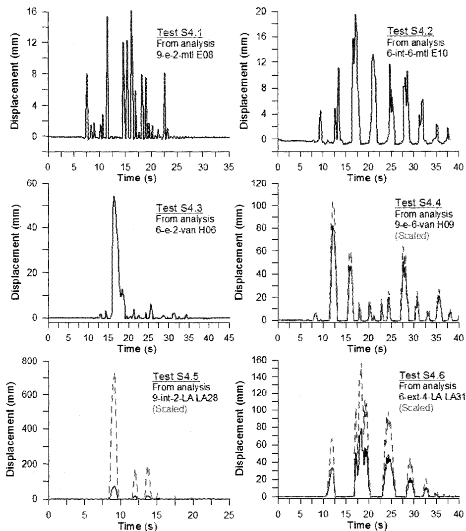
Figure 6.7: Displacement time history inputs used for test series 4.
