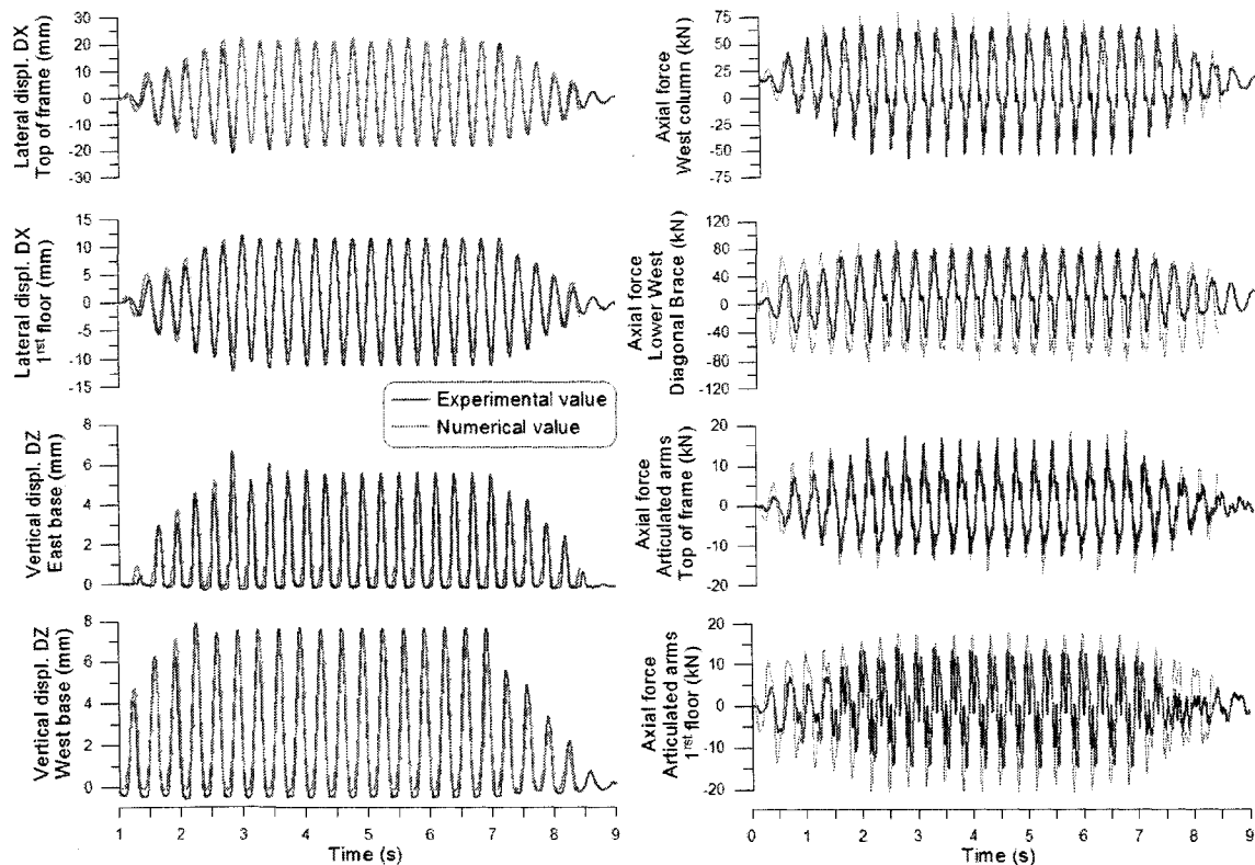
Figure 7.29: Comparison of the results for the ST1.26 input signal (Triangular 3Hz, 0.5g).
