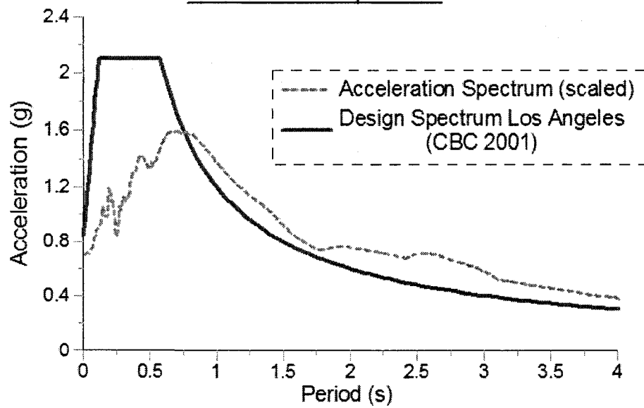
Acceleration - Spectrum
