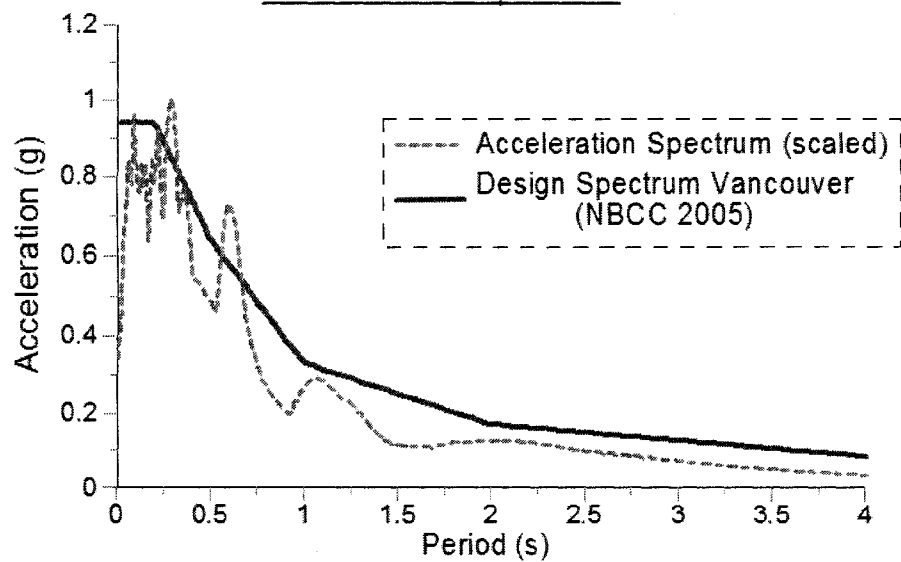
Acceleration - Spectrum
