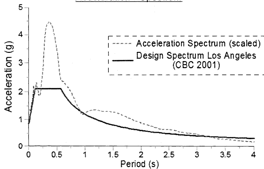
Acceleration - Spectrum
