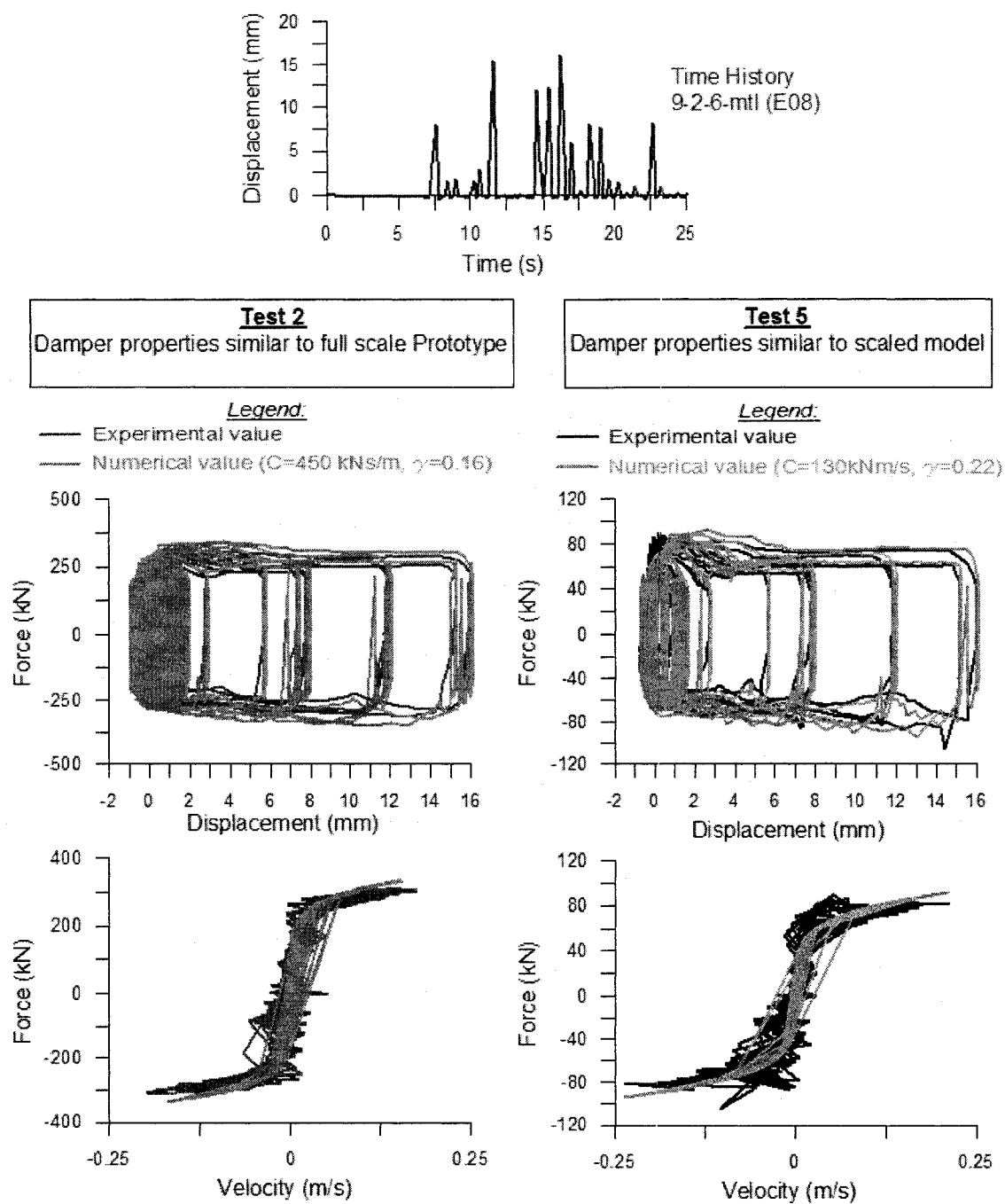
Figure 6.9: Input S4.1 – Time history displacement from parametric study Analysis: 9-2-6-mtl, Time history: E08
