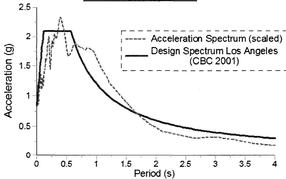
Acceleration - Spectrum
