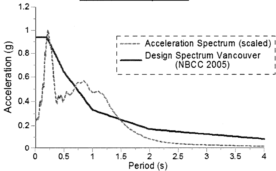
Acceleration - Spectrum
