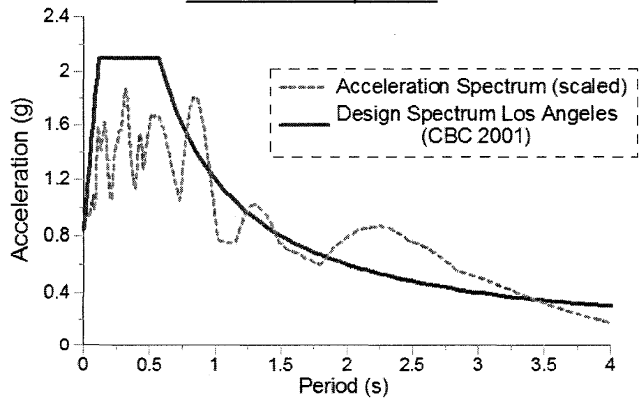
Acceleration - Spectrum
