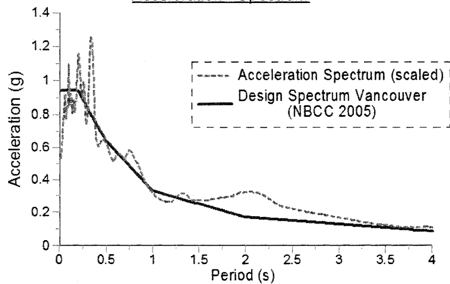
Acceleration - Spectrum
