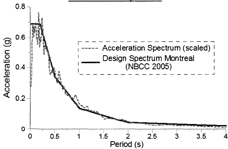
Acceleration - Spectrum
