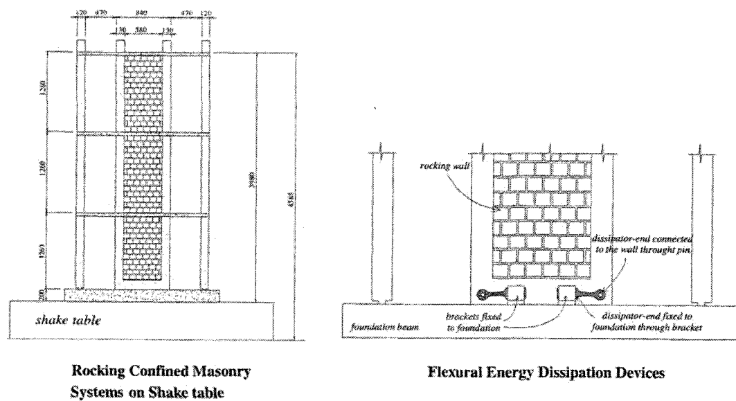
Figure 2.11: Test setup for the rocking confined masonry wall system (Toranzo et al., 2004).
