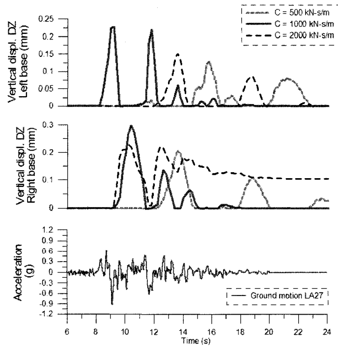
Figure 4.15: Rocking response of the 6-e-2-LA frame to the LA27 ground motion.
