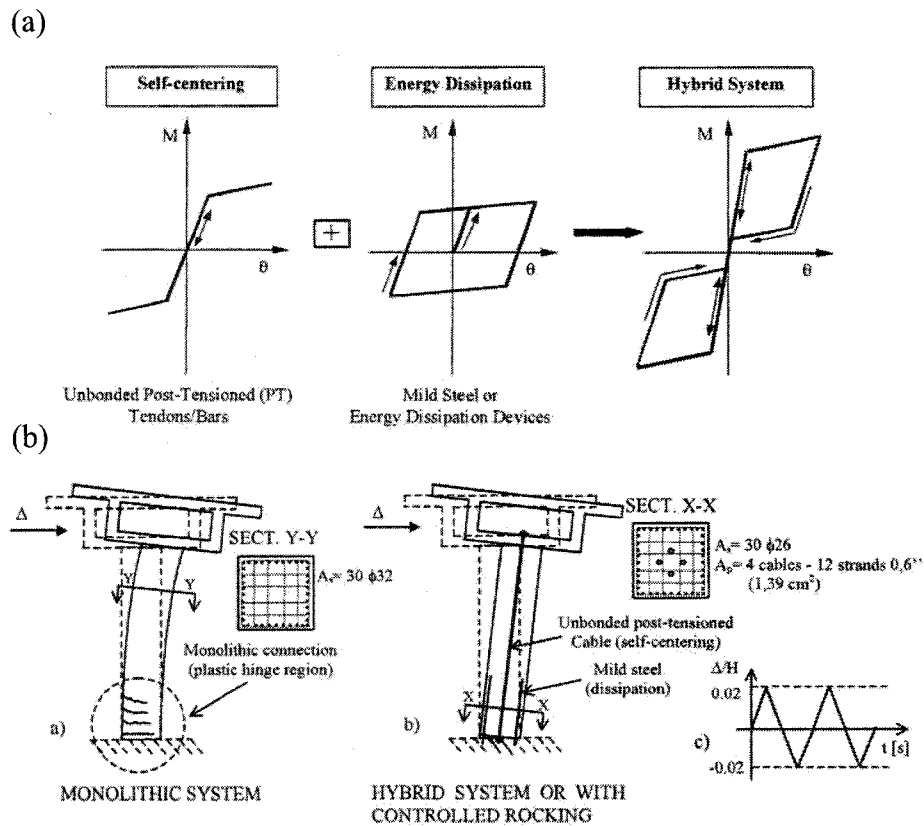
Figure 2.10: (a) Flag-shape hysteresis behaviour of the hybrid system (Palermo et al., 2004).
