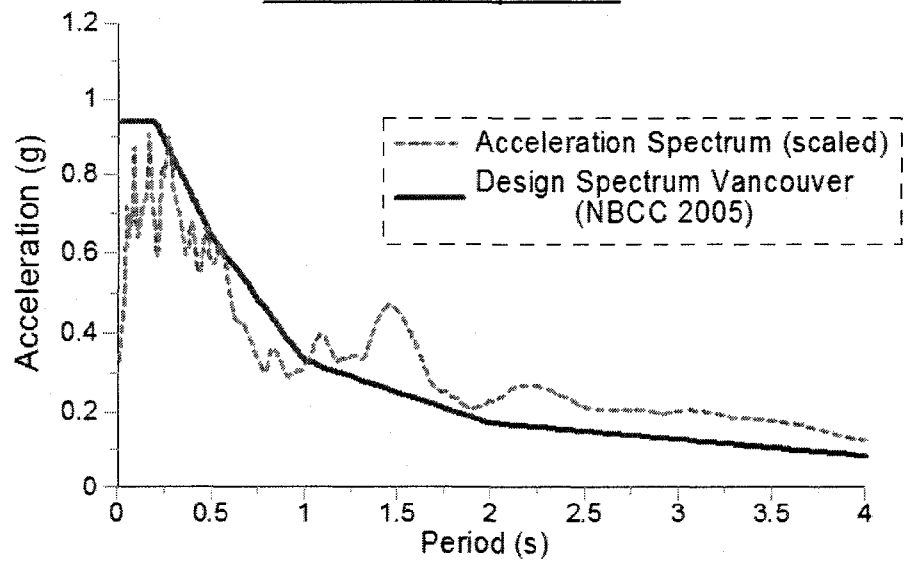
Acceleration - Spectrum
