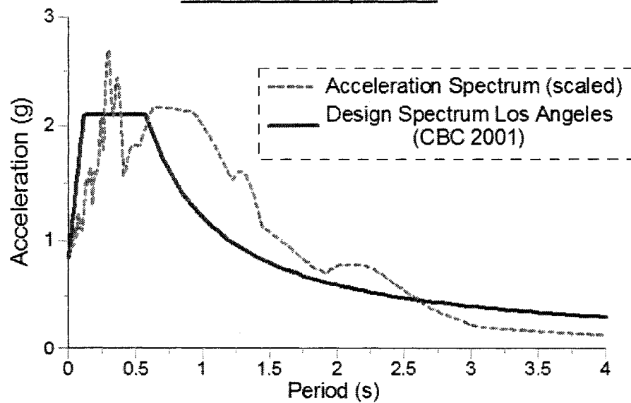
Acceleration - Spectrum
