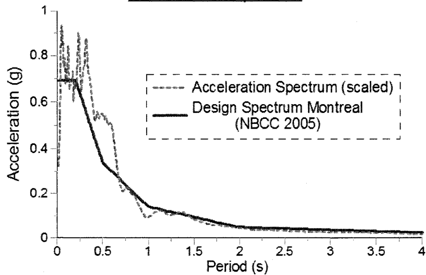
Acceleration - Spectrum
