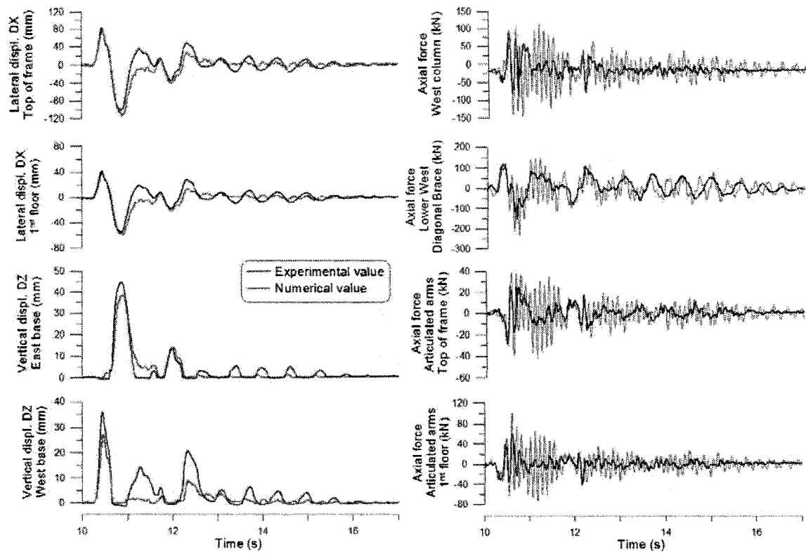
Figure 7.27: Comparison of the results for the ST1.7 input signal (Los Angeles, LA28).
