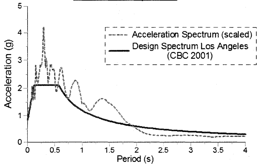
Acceleration - Spectrum
