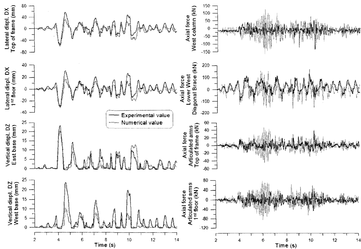
Figure 7.26: Comparison of the results for the STL.6 input signal (Vancouver, H09).
