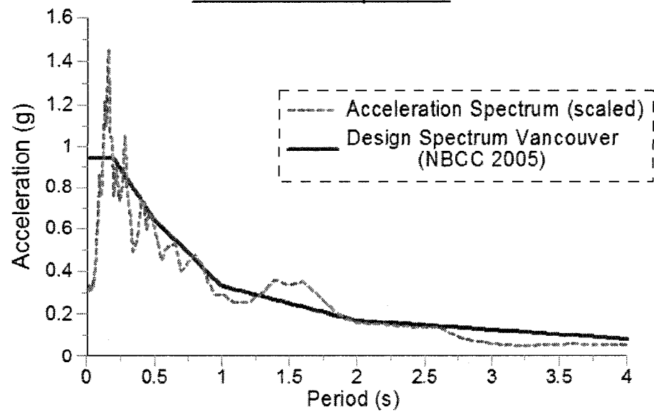
Acceleration - Spectrum
