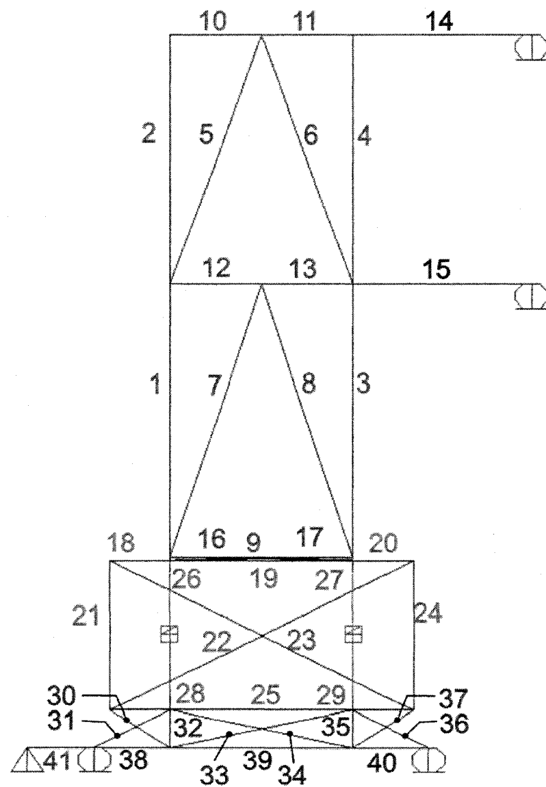
Figure H.1: Laboratory test specimen – Frame labels
