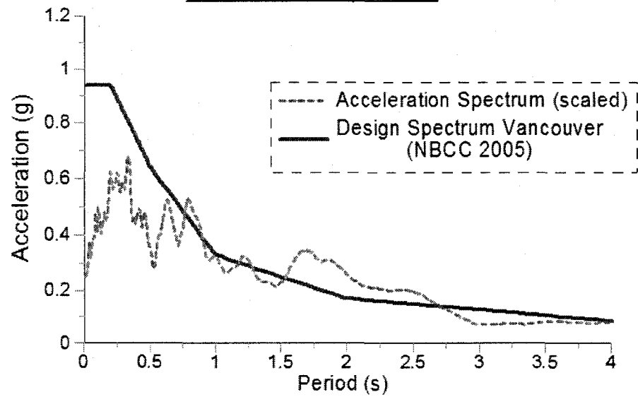
Acceleration - Spectrum
