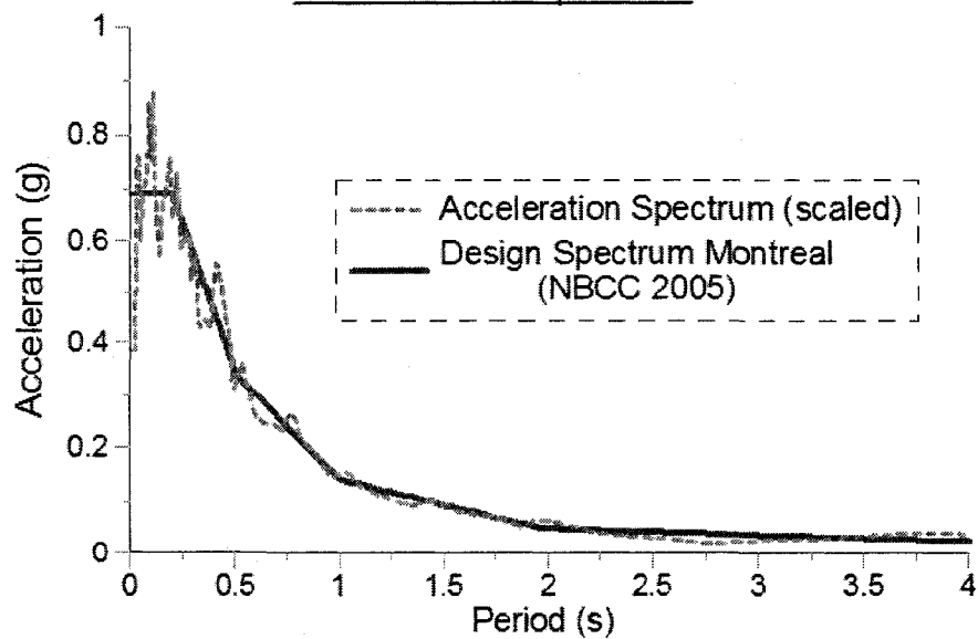
Acceleration - Spectrum
