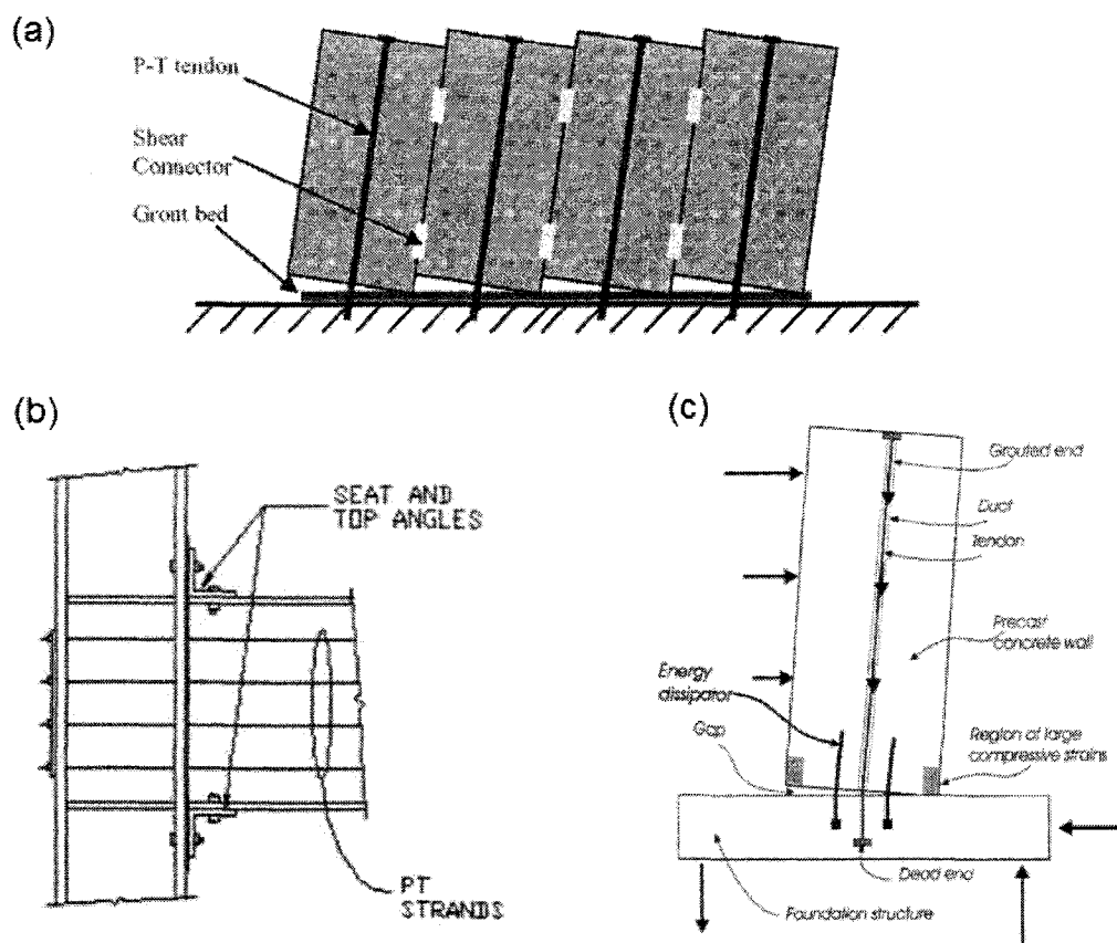
Figure 2.9: (a) Post-tensioned rocking wall system (Filiatrault et al., 2004).
