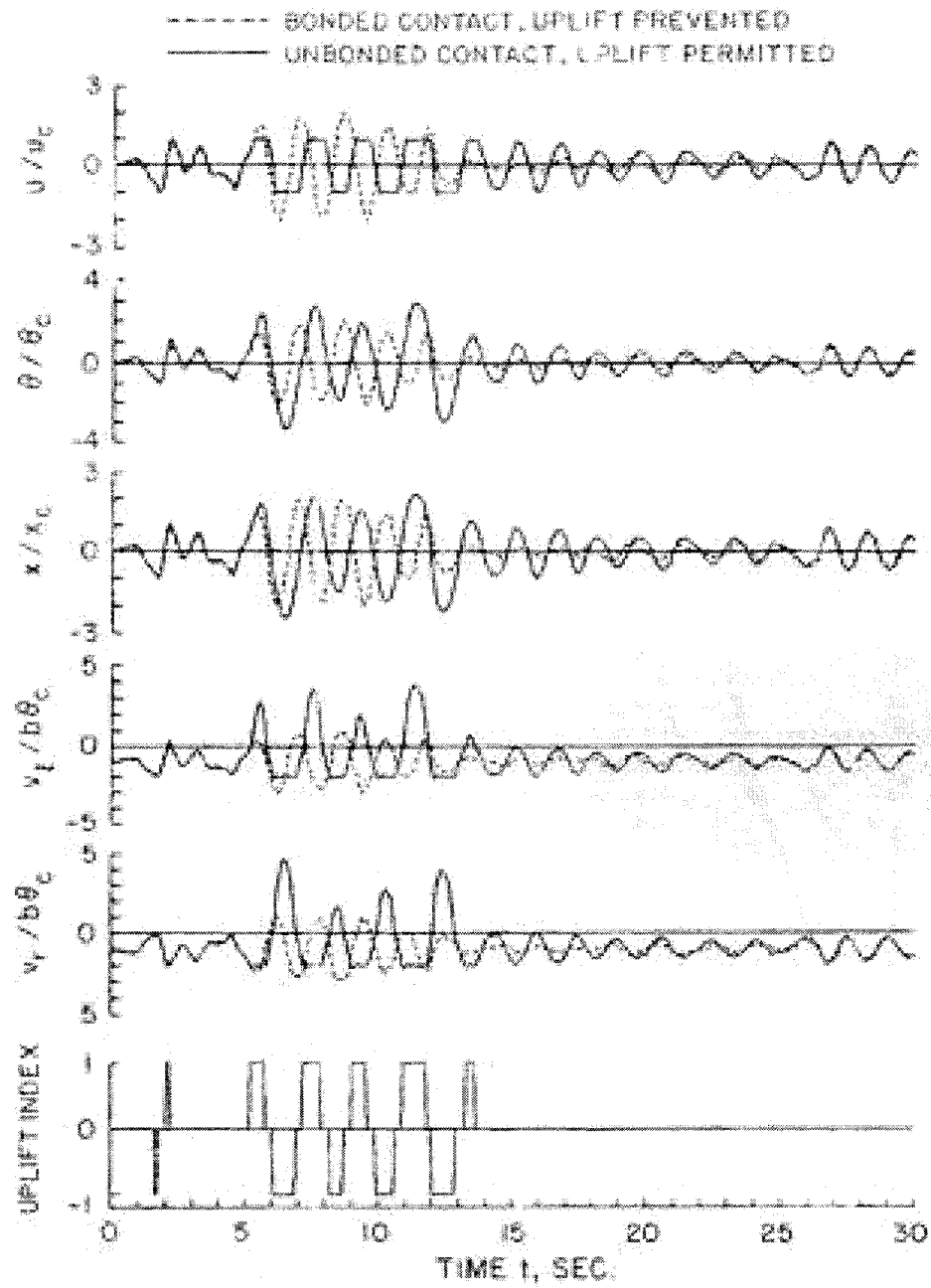
Figure 3.11: Analytical results – Earthquake response (Chopra and Yim, 1983).
