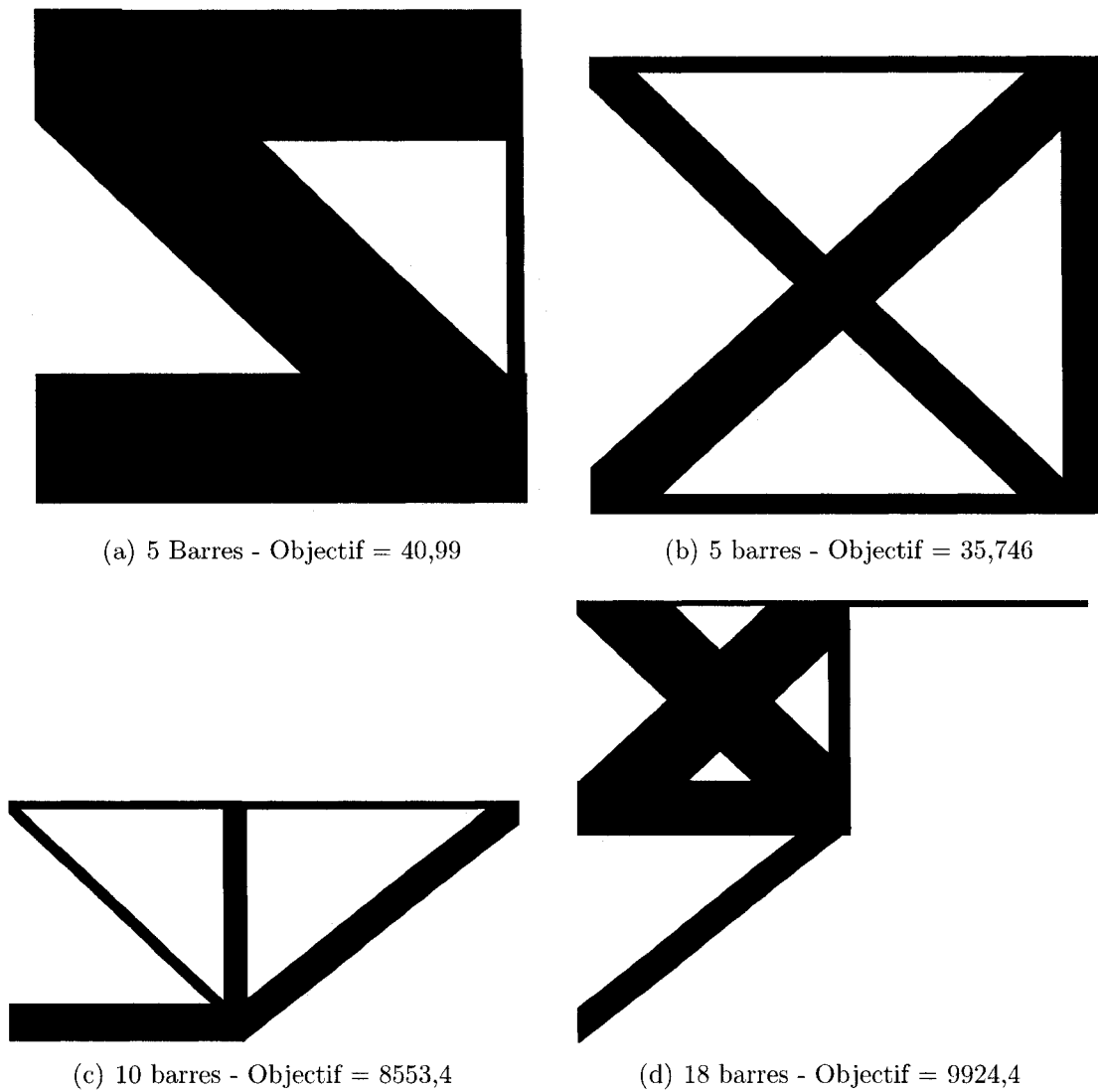
Figure 3.10 – Structures optimales
