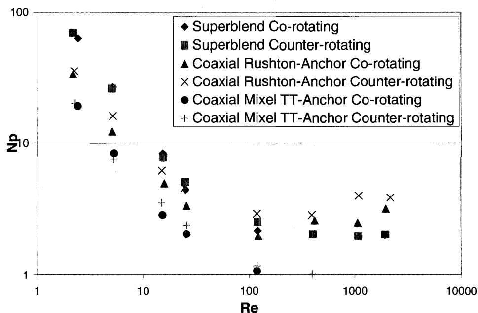
Figure 7-3 : Comparison of power curves between the Superblend and two configurations of a dual shaft coaxial mixer
