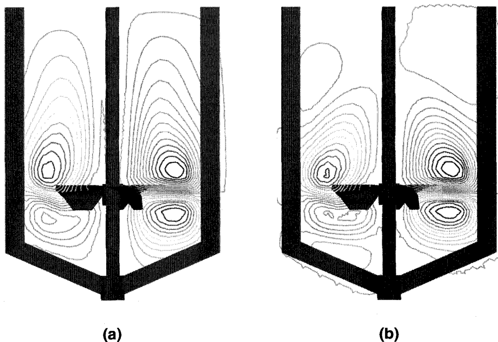
Figure 5-12 : Streamlines for the Mixel TT-anchor coaxial system in the XZ plane: (a): Co-rotating mode, Re = 130.5 ; (b): Counter-rotating mode, Re = 139.5
