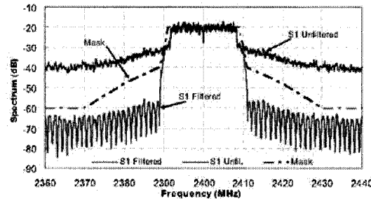
Fig. 3: Branch signal spectrum before and after filtering.
